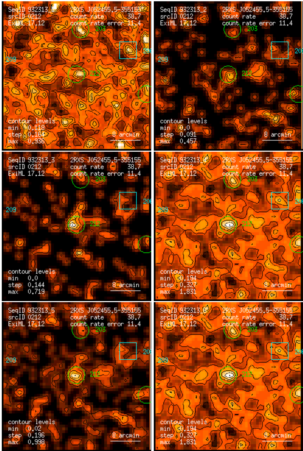
Figure 212: RASS 932313: detection 0212: band rate images, Gaussian filter: (1) PSPC channels 11 – 41, (2) 52 – 90, (3) 91 – 201, (4) 11 – 235, (5) 52 – 201, (6) 11 – 201. Broad band rates in counts/ks. Band rate contour levels in counts/ks/arcmin 2 .
