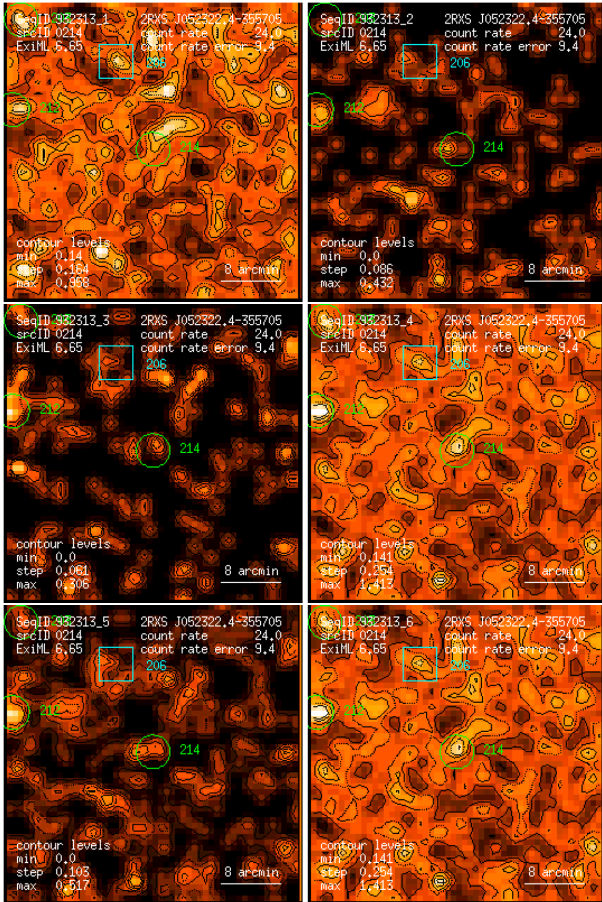
Figure 214: RASS 932313: detection 0214: band rate images, Gaussian filter: (1) PSPC channels 11 – 41, (2) 52 – 90, (3) 91 – 201, (4) 11 – 235, (5) 52 – 201, (6) 11 – 201. Broad band rates in counts/ks. Band rate contour levels in counts/ks/arcmin 2 .
