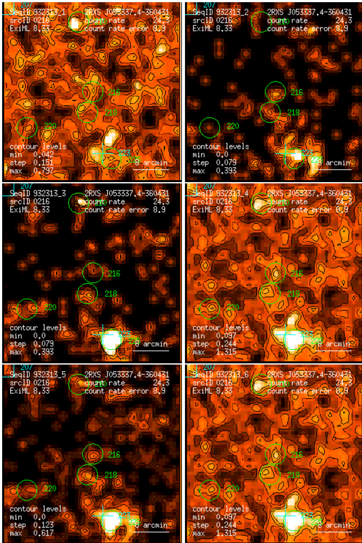
Figure 216: RASS 932313: detection 0216: band rate images, Gaussian filter: (1) PSPC channels 11 – 41, (2) 52 – 90, (3) 91 – 201, (4) 11 – 235, (5) 52 – 201, (6) 11 – 201. Broad band rates in counts/ks. Band rate contour levels in counts/ks/arcmin 2 .
