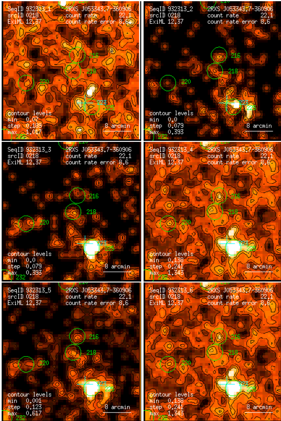
Figure 218: RASS 932313: detection 0218: band rate images, Gaussian filter: (1) PSPC channels 11 – 41, (2) 52 – 90, (3) 91 – 201, (4) 11 – 235, (5) 52 – 201, (6) 11 – 201. Broad band rates in counts/ks. Band rate contour levels in counts/ks/arcmin 2 .
