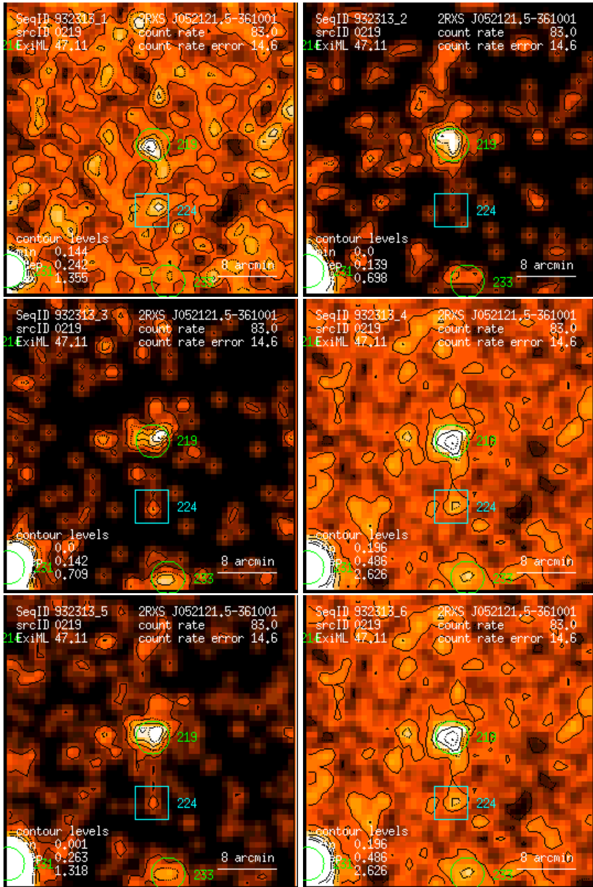
Figure 219: RASS 932313: detection 0219: band rate images, Gaussian filter: (1) PSPC channels 11 – 41, (2) 52 – 90, (3) 91 – 201, (4) 11 – 235, (5) 52 – 201, (6) 11 – 201. Broad band rates in counts/ks. Band rate contour levels in counts/ks/arcmin 2 .
