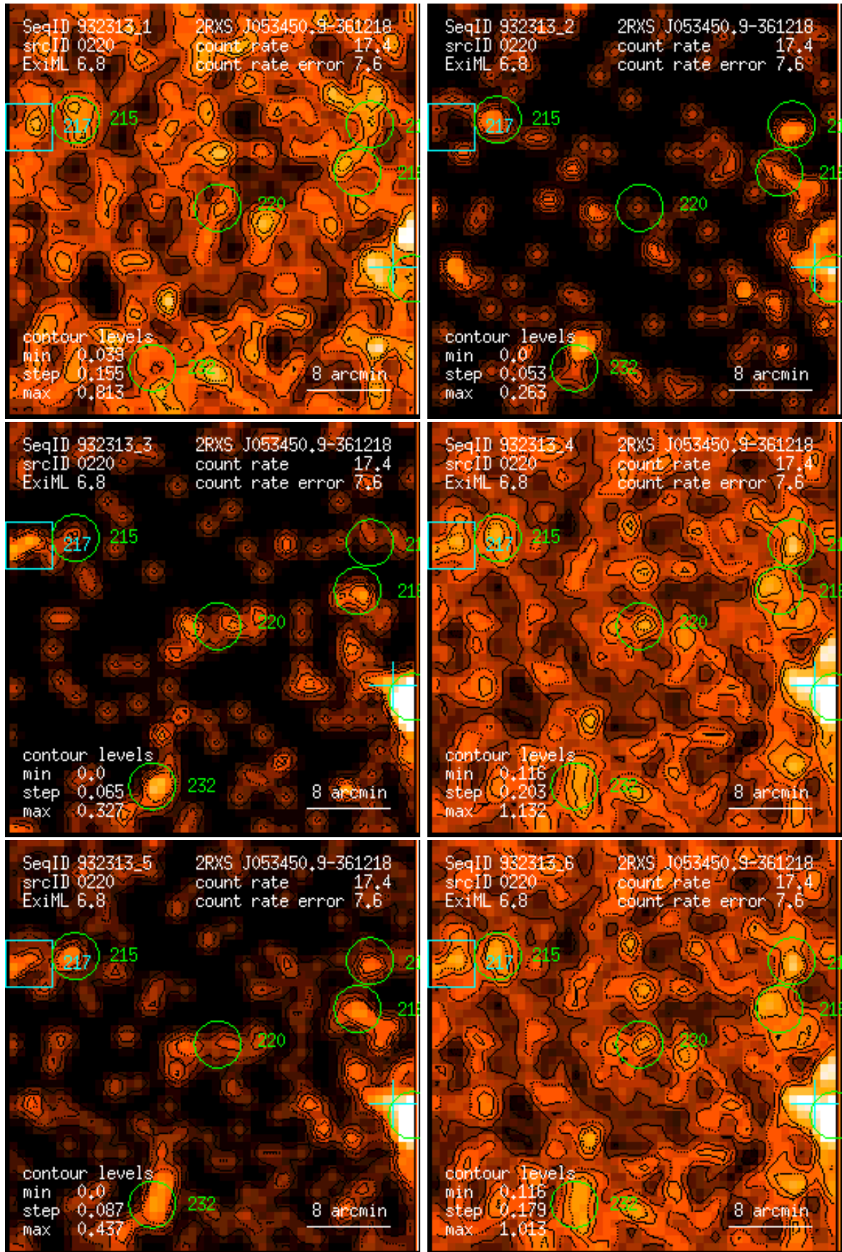
Figure 220: RASS 932313: detection 0220: band rate images, Gaussian filter: (1) PSPC channels 11 – 41, (2) 52 – 90, (3) 91 – 201, (4) 11 – 235, (5) 52 – 201, (6) 11 – 201. Broad band rates in counts/ks. Band rate contour levels in counts/ks/arcmin 2 .
