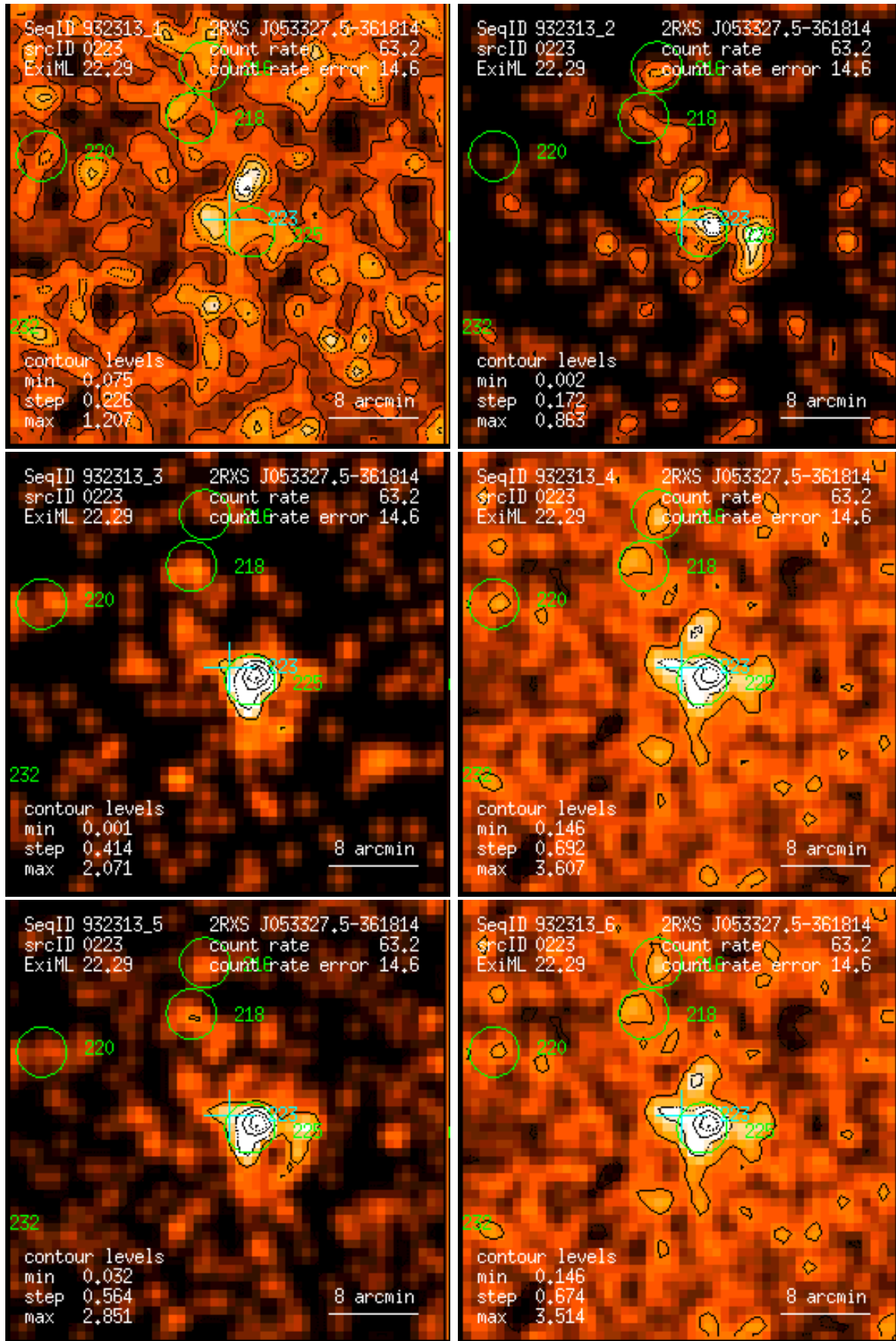
Figure 223: RASS 932313: detection 0223: band rate images, Gaussian filter: (1) PSPC channels 11 – 41, (2) 52 – 90, (3) 91 – 201, (4) 11 – 235, (5) 52 – 201, (6) 11 – 201. Broad band rates in counts/ks. Band rate contour levels in counts/ks/arcmin 2 .
