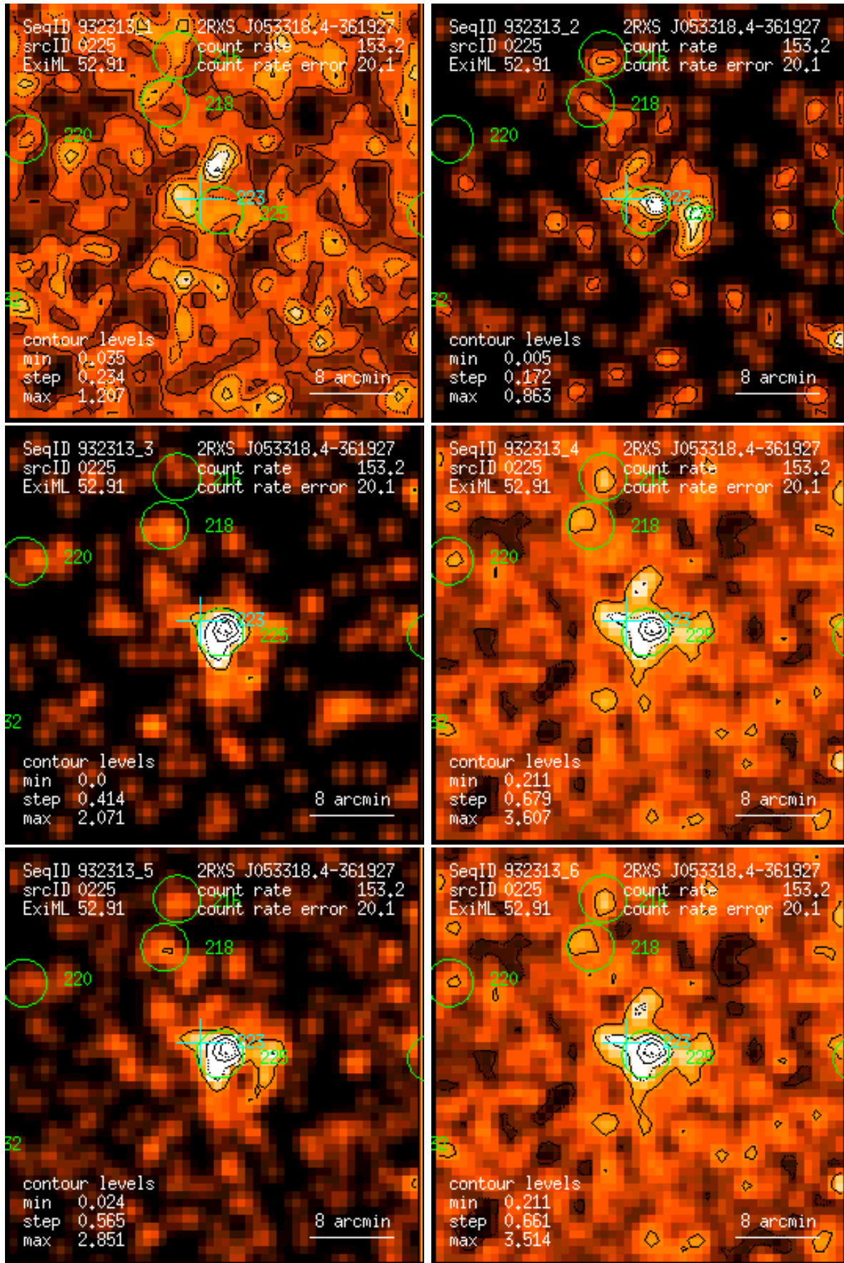
Figure 225: RASS 932313: detection 0225: band rate images, Gaussian filter: (1) PSPC channels 11 – 41, (2) 52 – 90, (3) 91 – 201, (4) 11 – 235, (5) 52 – 201, (6) 11 – 201. Broad band rates in counts/ks. Band rate contour levels in counts/ks/arcmin 2 .
