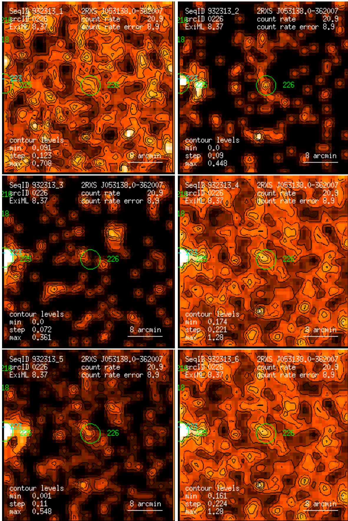
Figure 226: RASS 932313: detection 0226: band rate images, Gaussian filter: (1) PSPC channels 11 – 41, (2) 52 – 90, (3) 91 – 201, (4) 11 – 235, (5) 52 – 201, (6) 11 – 201. Broad band rates in counts/ks. Band rate contour levels in counts/ks/arcmin 2 .
