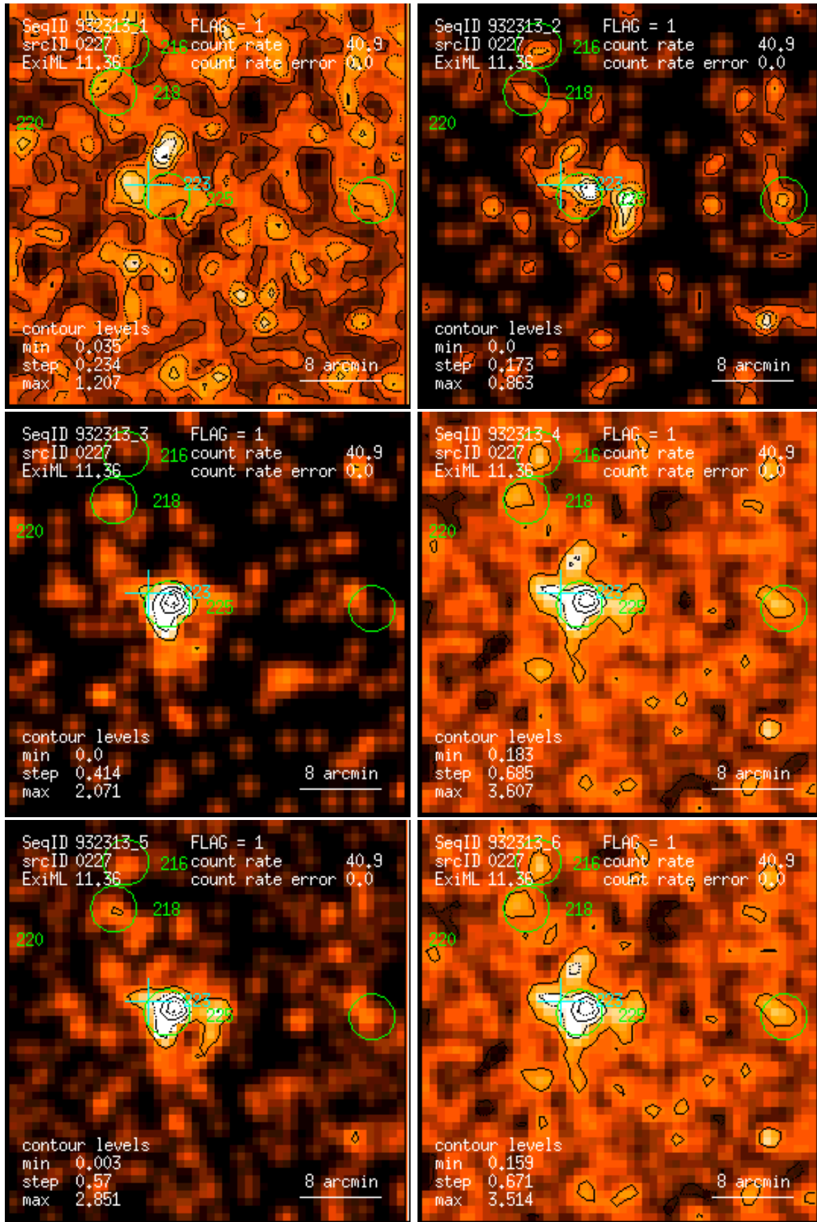
Figure 227: RASS 932313: detection 0227: band rate images, Gaussian filter: (1) PSPC channels 11 – 41, (2) 52 – 90, (3) 91 – 201, (4) 11 – 235, (5) 52 – 201, (6) 11 – 201. Broad band rates in counts/ks. Band rate contour levels in counts/ks/arcmin 2 .
