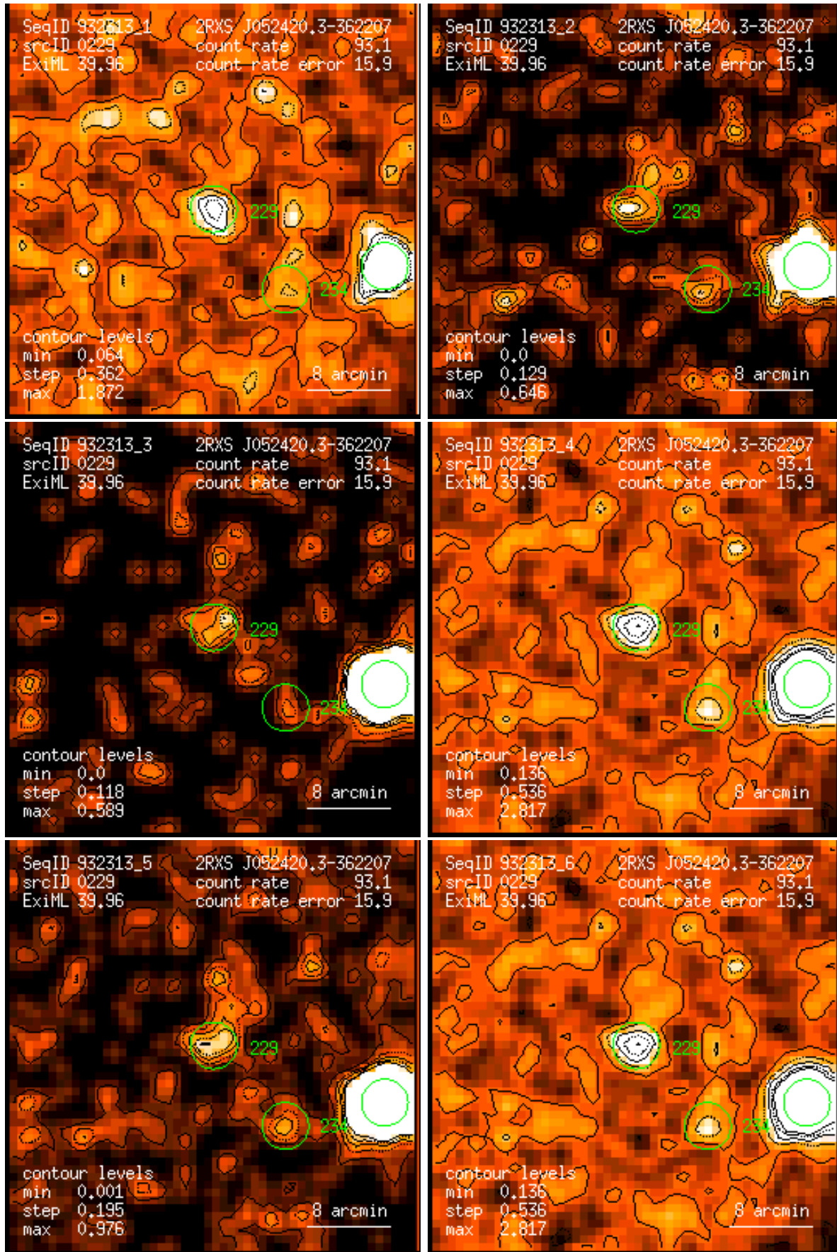
Figure 229: RASS 932313: detection 0229: band rate images, Gaussian filter: (1) PSPC channels 11 – 41, (2) 52 – 90, (3) 91 – 201, (4) 11 – 235, (5) 52 – 201, (6) 11 – 201. Broad band rates in counts/ks. Band rate contour levels in counts/ks/arcmin 2 .
