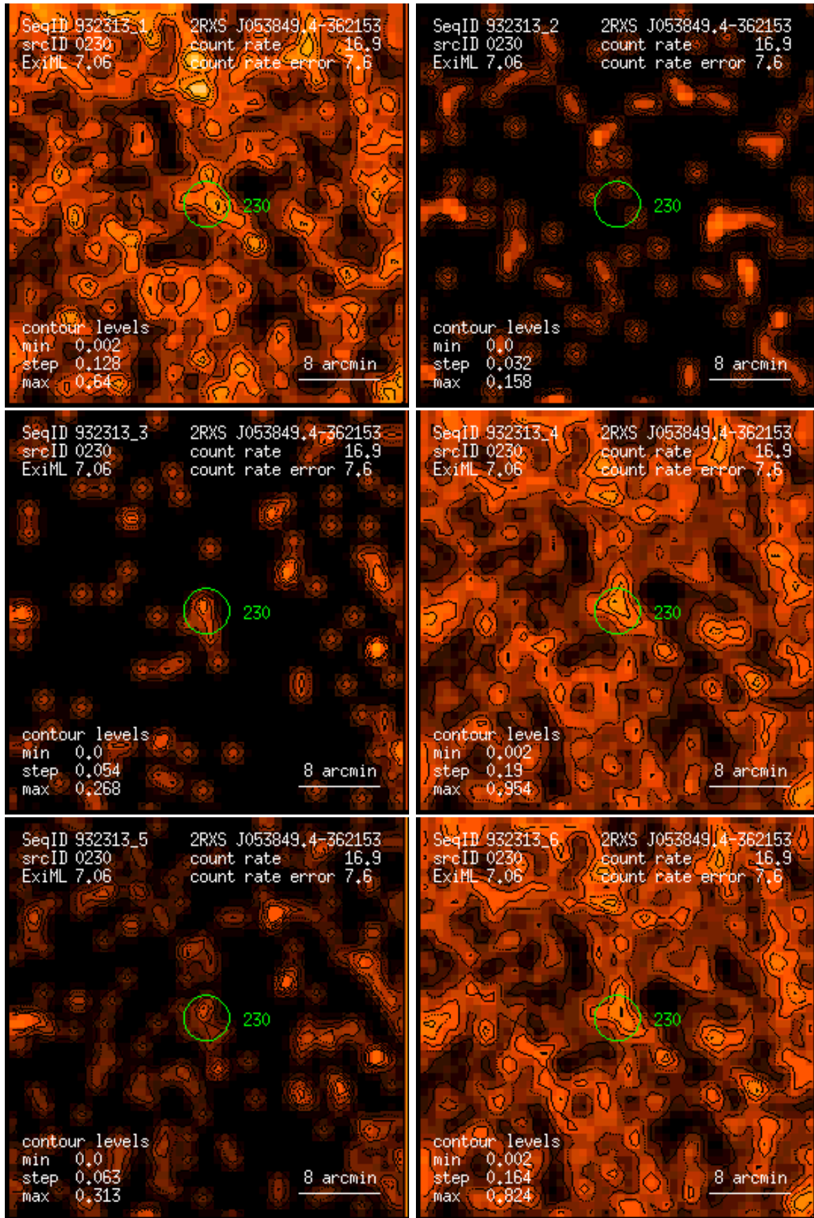
Figure 230: RASS 932313: detection 0230: band rate images, Gaussian filter: (1) PSPC channels 11 – 41, (2) 52 – 90, (3) 91 – 201, (4) 11 – 235, (5) 52 – 201, (6) 11 – 201. Broad band rates in counts/ks. Band rate contour levels in counts/ks/arcmin 2 .
