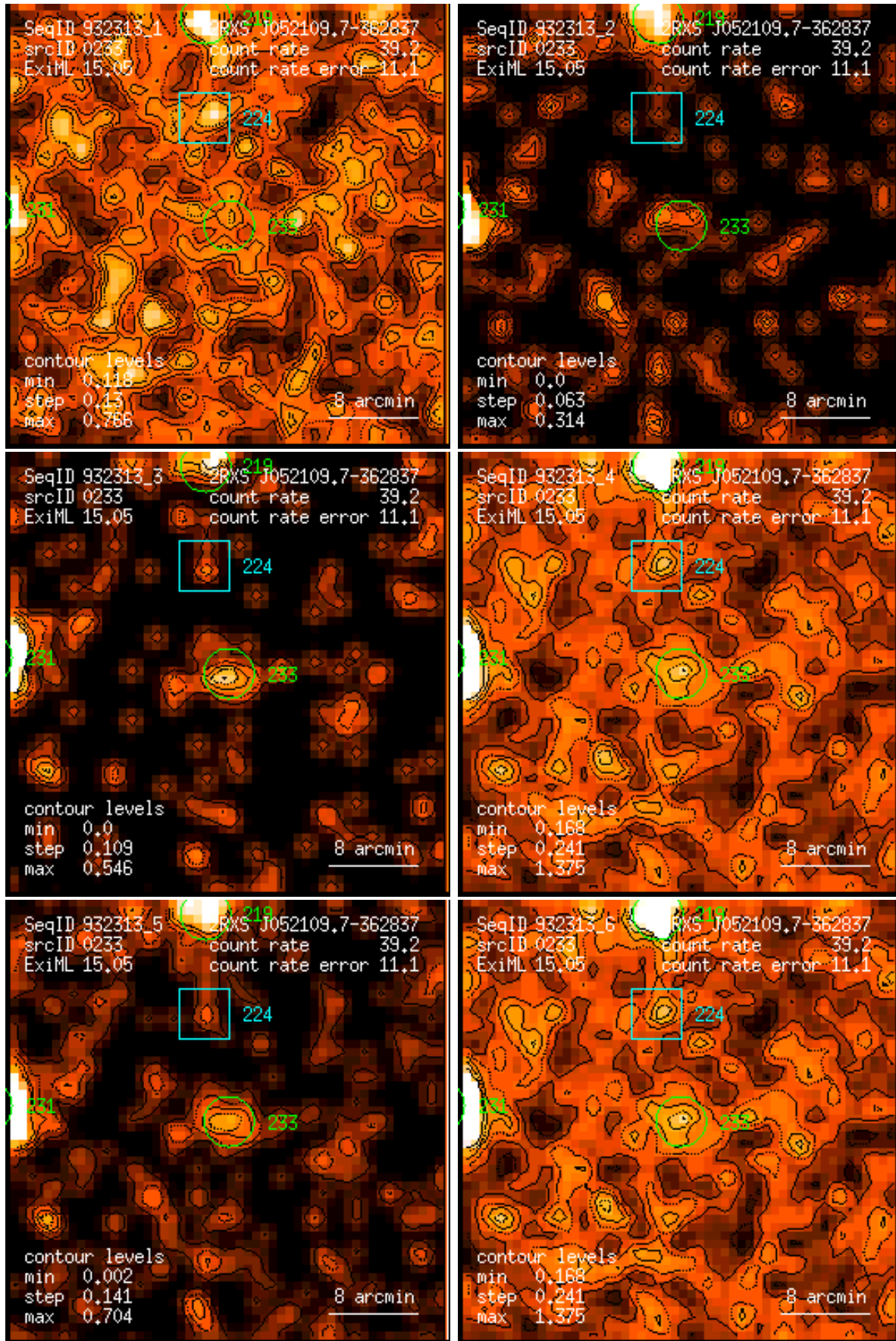
Figure 233: RASS 932313: detection 0233: band rate images, Gaussian filter: (1) PSPC channels 11 – 41, (2) 52 – 90, (3) 91 – 201, (4) 11 – 235, (5) 52 – 201, (6) 11 – 201. Broad band rates in counts/ks. Band rate contour levels in counts/ks/arcmin 2 .
