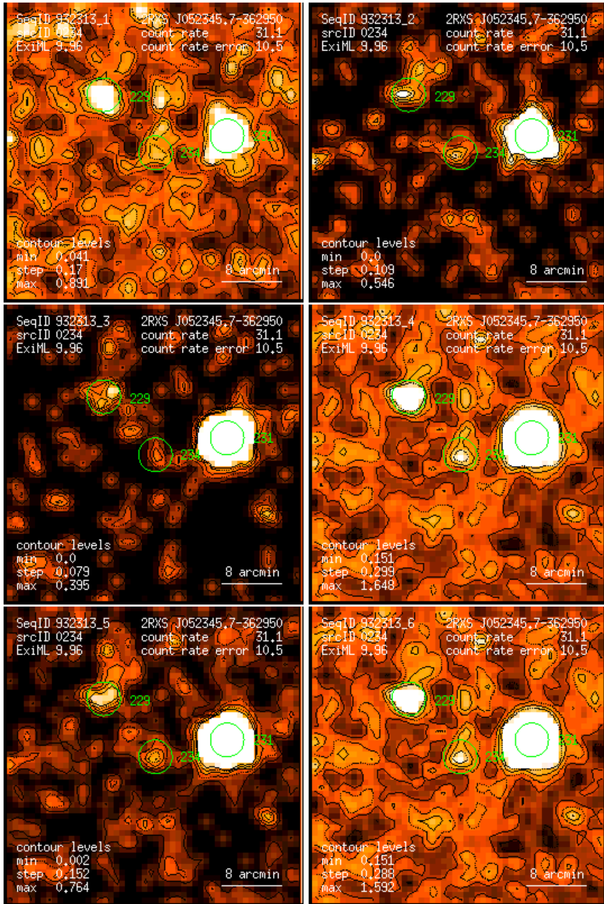
Figure 234: RASS 932313: detection 0234: band rate images, Gaussian filter: (1) PSPC channels 11 – 41, (2) 52 – 90, (3) 91 – 201, (4) 11 – 235, (5) 52 – 201, (6) 11 – 201. Broad band rates in counts/ks. Band rate contour levels in counts/ks/arcmin 2 .
