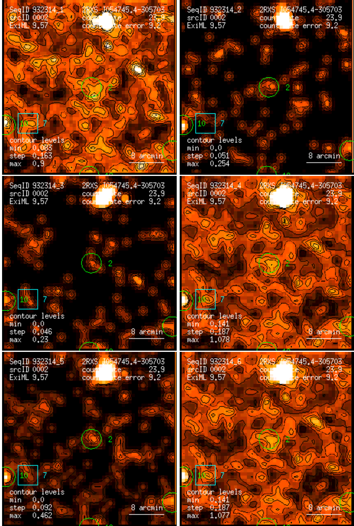
Figure 2: RASS 932314: detection 0002: band rate images, Gaussian filter: (1) PSPC channels 11 – 41, (2) 52 – 90, (3) 91 – 201, (4) 11 – 235, (5) 52 – 201, (6) 11 – 201. Broad band rates in counts/ks. Band rate contour levels in counts/ks/arcmin 2 .
