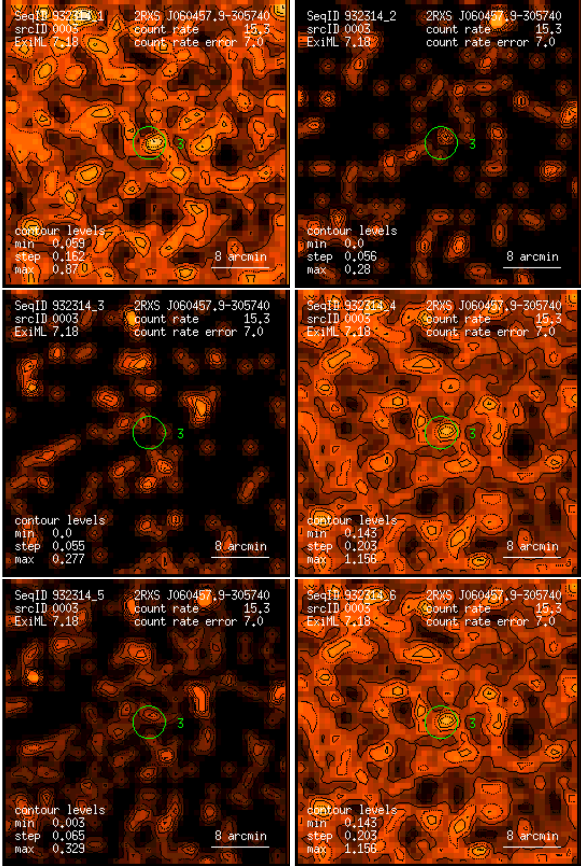
Figure 3: RASS 932314: detection 0003: band rate images, Gaussian filter: (1) PSPC channels 11 – 41, (2) 52 – 90, (3) 91 – 201, (4) 11 – 235, (5) 52 – 201, (6) 11 – 201. Broad band rates in counts/ks. Band rate contour levels in counts/ks/arcmin 2 .
