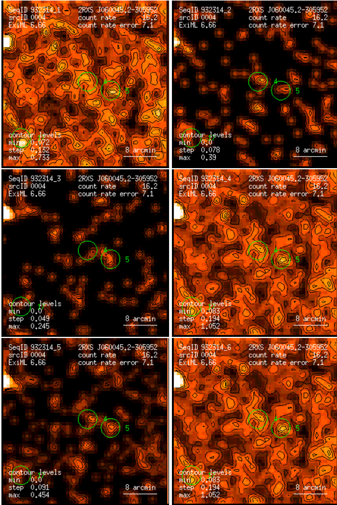
Figure 4: RASS 932314: detection 0004: band rate images, Gaussian filter: (1) PSPC channels 11 – 41, (2) 52 – 90, (3) 91 – 201, (4) 11 – 235, (5) 52 – 201, (6) 11 – 201. Broad band rates in counts/ks. Band rate contour levels in counts/ks/arcmin 2 .
