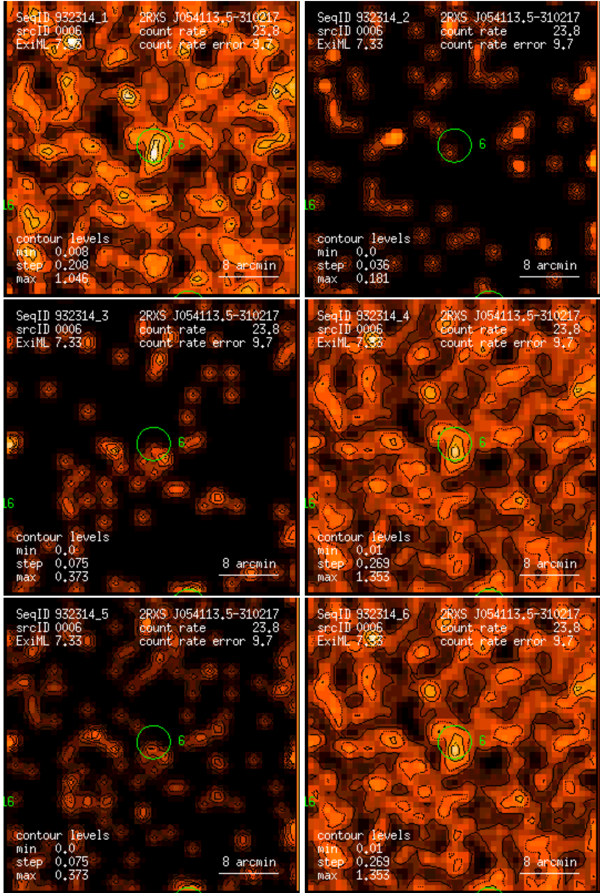
Figure 6: RASS 932314: detection 0006: band rate images, Gaussian filter: (1) PSPC channels 11 – 41, (2) 52 – 90, (3) 91 – 201, (4) 11 – 235, (5) 52 – 201, (6) 11 – 201. Broad band rates in counts/ks. Band rate contour levels in counts/ks/arcmin 2 .
