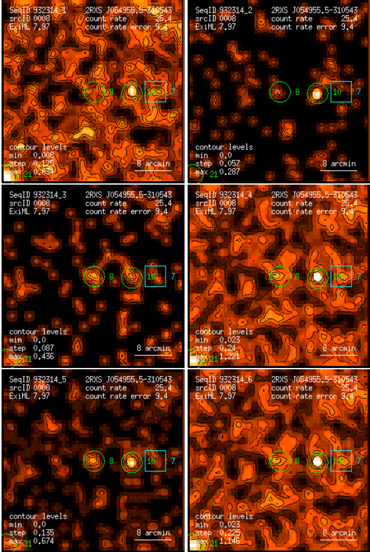
Figure 8: RASS 932314: detection 0008: band rate images, Gaussian filter: (1) PSPC channels 11 – 41, (2) 52 – 90, (3) 91 – 201, (4) 11 – 235, (5) 52 – 201, (6) 11 – 201. Broad band rates in counts/ks. Band rate contour levels in counts/ks/arcmin 2 .
