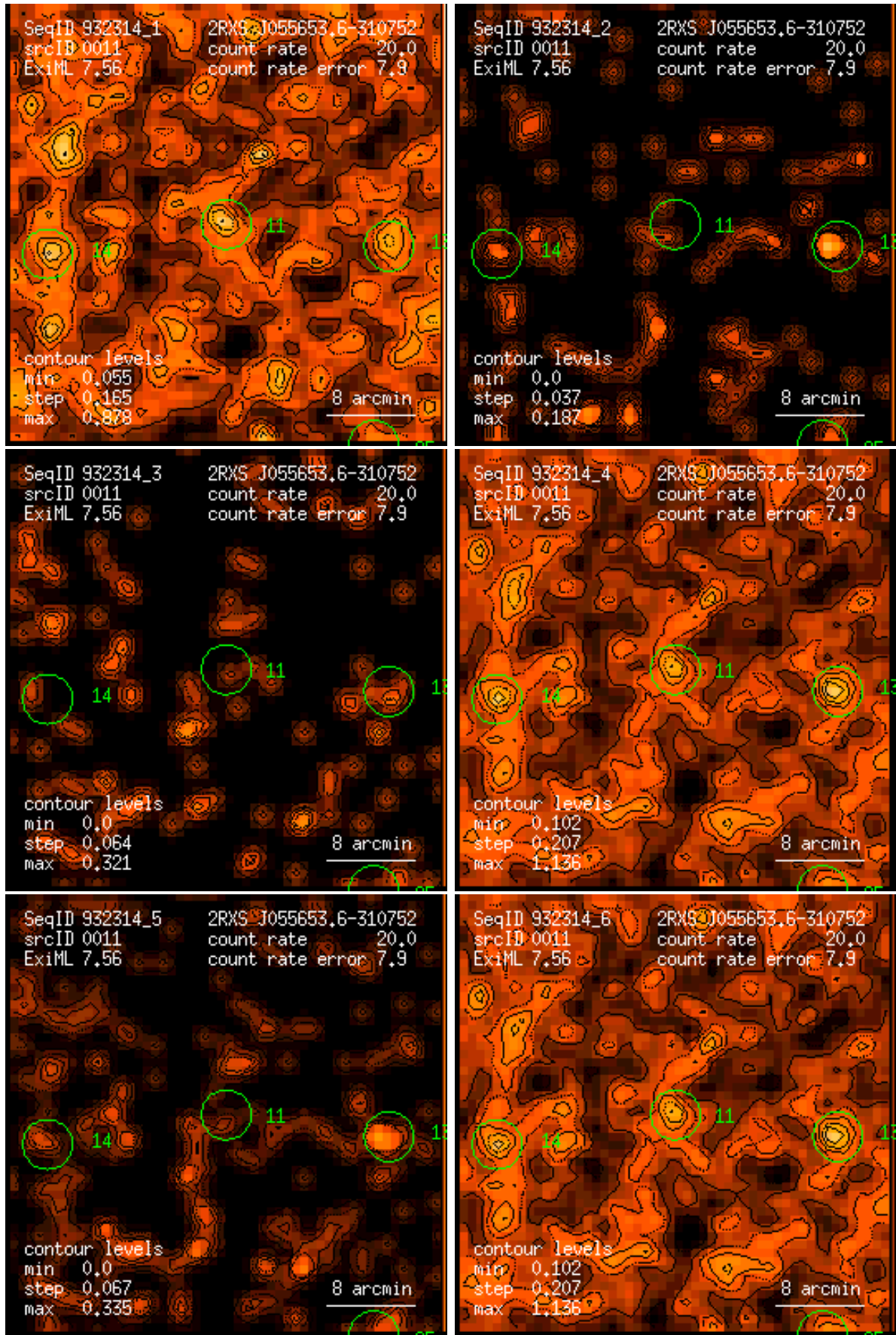
Figure 11: RASS 932314: detection 0011: band rate images, Gaussian filter: (1) PSPC channels 11 – 41, (2) 52 – 90, (3) 91 – 201, (4) 11 – 235, (5) 52 – 201, (6) 11 – 201. Broad band rates in counts/ks. Band rate contour levels in counts/ks/arcmin 2 .
