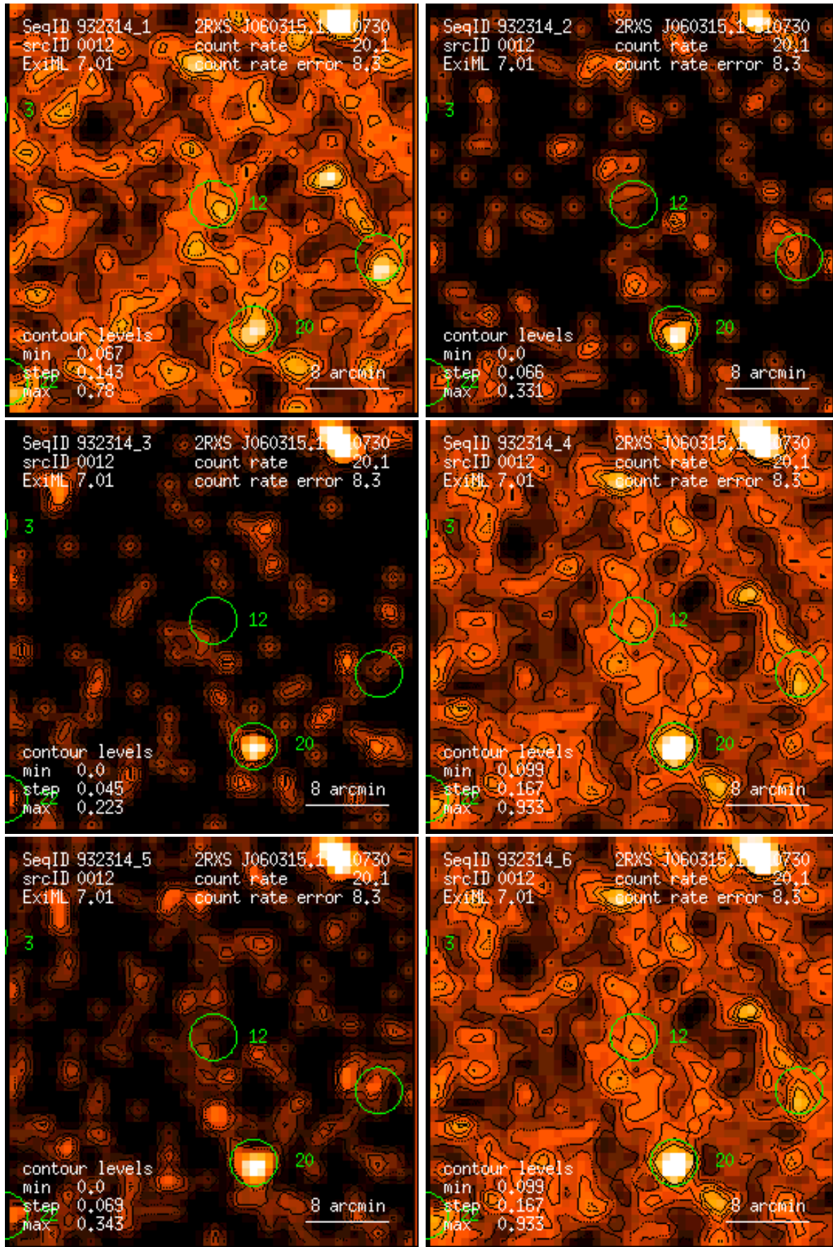
Figure 12: RASS 932314: detection 0012: band rate images, Gaussian filter: (1) PSPC channels 11 – 41, (2) 52 – 90, (3) 91 – 201, (4) 11 – 235, (5) 52 – 201, (6) 11 – 201. Broad band rates in counts/ks. Band rate contour levels in counts/ks/arcmin 2 .
