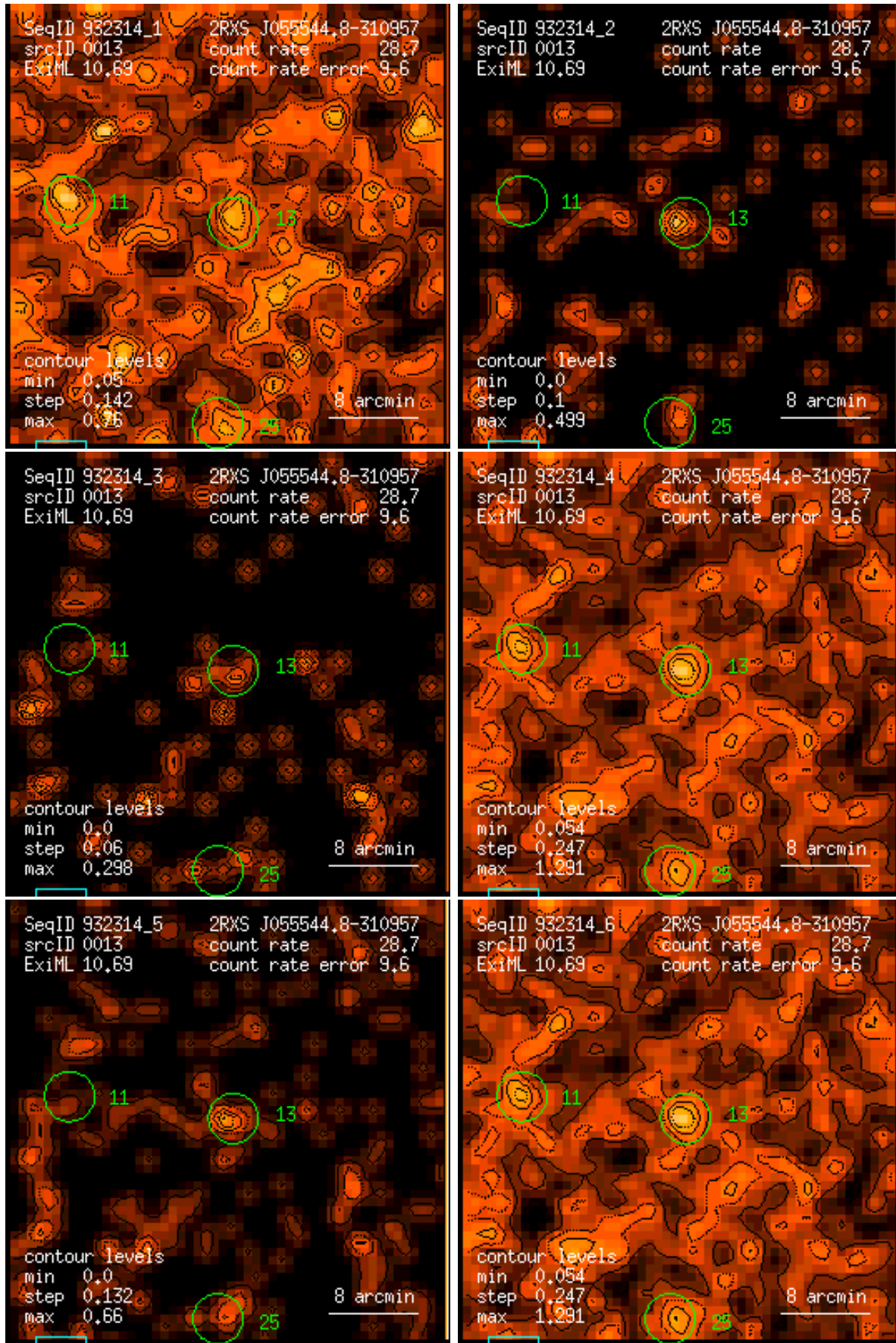
Figure 13: RASS 932314: detection 0013: band rate images, Gaussian filter: (1) PSPC channels 11 – 41, (2) 52 – 90, (3) 91 – 201, (4) 11 – 235, (5) 52 – 201, (6) 11 – 201. Broad band rates in counts/ks. Band rate contour levels in counts/ks/arcmin 2 .
