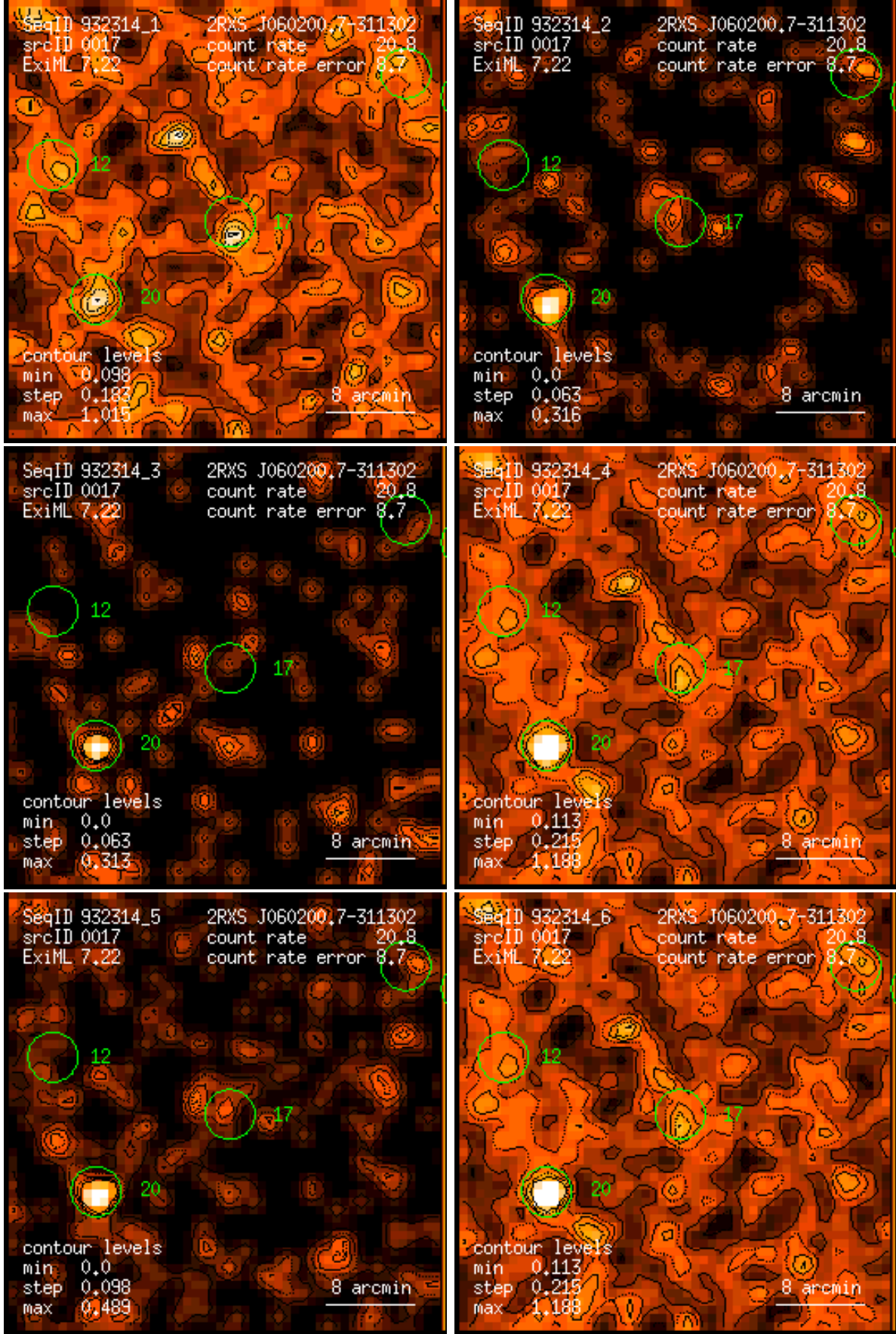
Figure 17: RASS 932314: detection 0017: band rate images, Gaussian filter: (1) PSPC channels 11 – 41, (2) 52 – 90, (3) 91 – 201, (4) 11 – 235, (5) 52 – 201, (6) 11 – 201. Broad band rates in counts/ks. Band rate contour levels in counts/ks/arcmin 2 .
