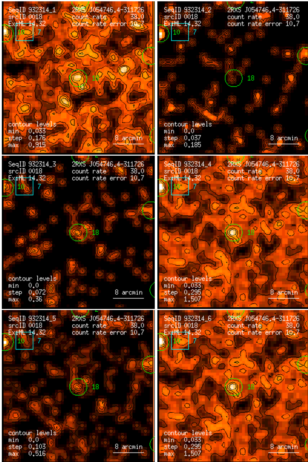
Figure 18: RASS 932314: detection 0018: band rate images, Gaussian filter: (1) PSPC channels 11 – 41, (2) 52 – 90, (3) 91 – 201, (4) 11 – 235, (5) 52 – 201, (6) 11 – 201. Broad band rates in counts/ks. Band rate contour levels in counts/ks/arcmin 2 .
