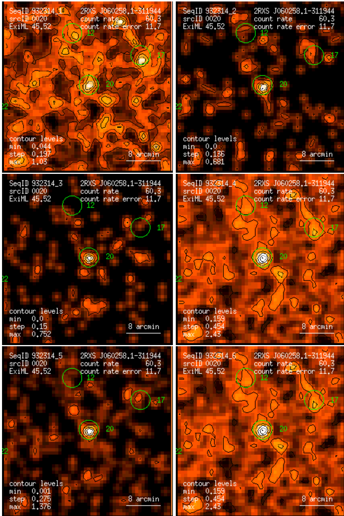
Figure 20: RASS 932314: detection 0020: band rate images, Gaussian filter: (1) PSPC channels 11 – 41, (2) 52 – 90, (3) 91 – 201, (4) 11 – 235, (5) 52 – 201, (6) 11 – 201. Broad band rates in counts/ks. Band rate contour levels in counts/ks/arcmin 2 .
