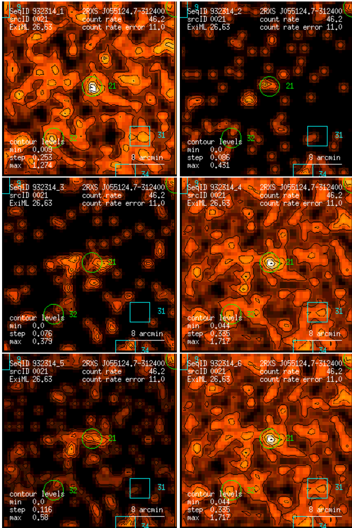
Figure 21: RASS 932314: detection 0021: band rate images, Gaussian filter: (1) PSPC channels 11 – 41, (2) 52 – 90, (3) 91 – 201, (4) 11 – 235, (5) 52 – 201, (6) 11 – 201. Broad band rates in counts/ks. Band rate contour levels in counts/ks/arcmin 2 .
