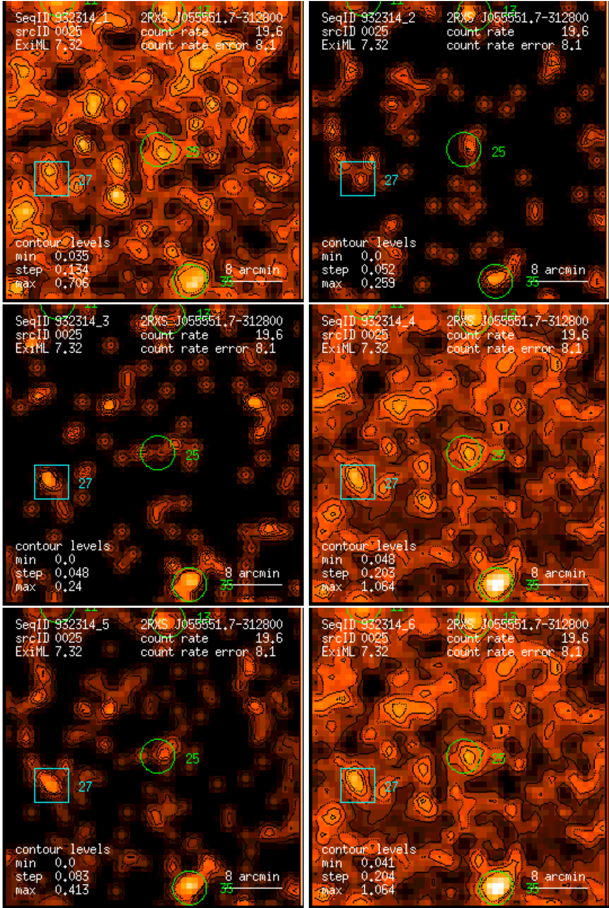
Figure 25: RASS 932314: detection 0025: band rate images, Gaussian filter: (1) PSPC channels 11 – 41, (2) 52 – 90, (3) 91 – 201, (4) 11 – 235, (5) 52 – 201, (6) 11 – 201. Broad band rates in counts/ks. Band rate contour levels in counts/ks/arcmin 2 .
