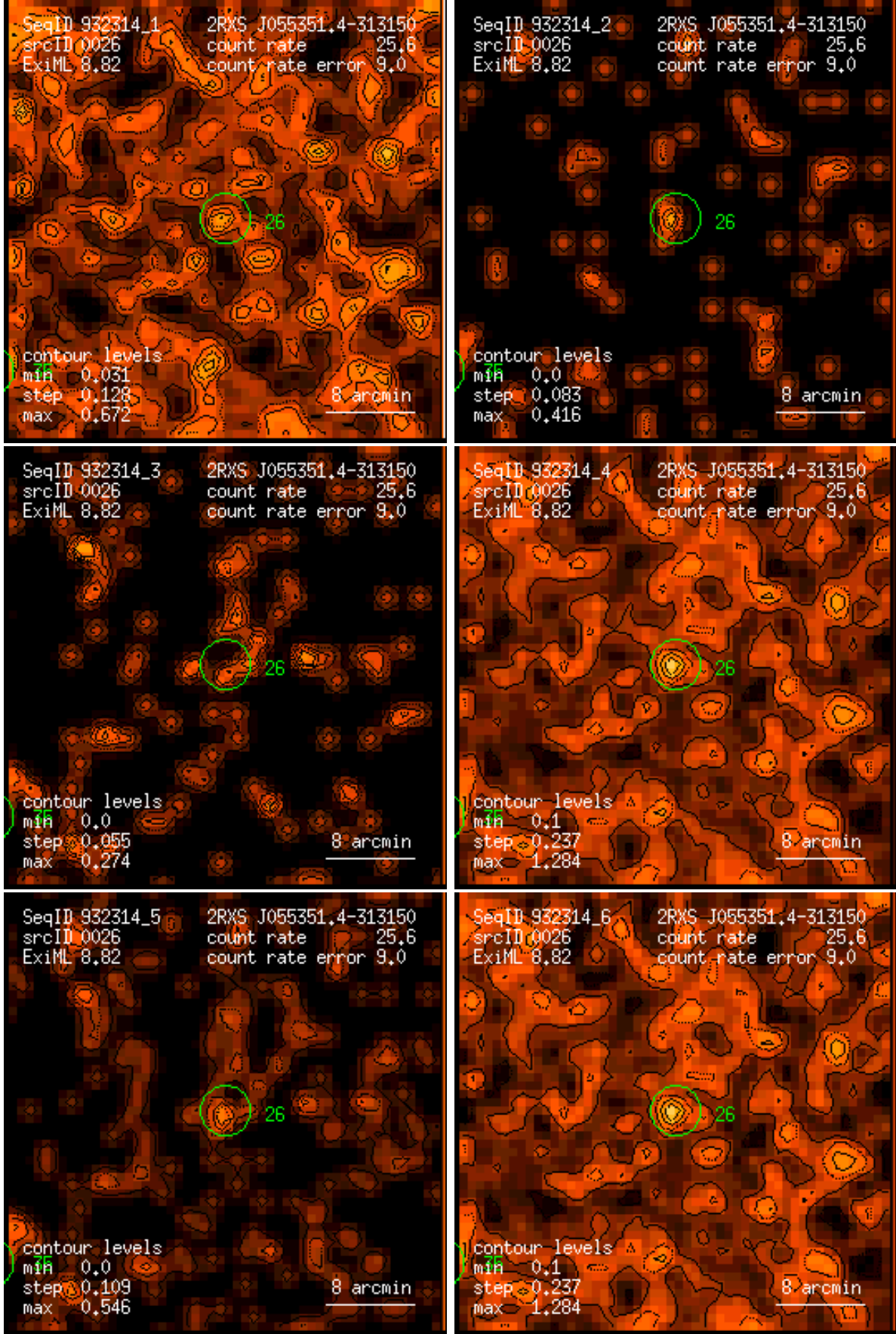
Figure 26: RASS 932314: detection 0026: band rate images, Gaussian filter: (1) PSPC channels 11 – 41, (2) 52 – 90, (3) 91 – 201, (4) 11 – 235, (5) 52 – 201, (6) 11 – 201. Broad band rates in counts/ks. Band rate contour levels in counts/ks/arcmin 2 .
