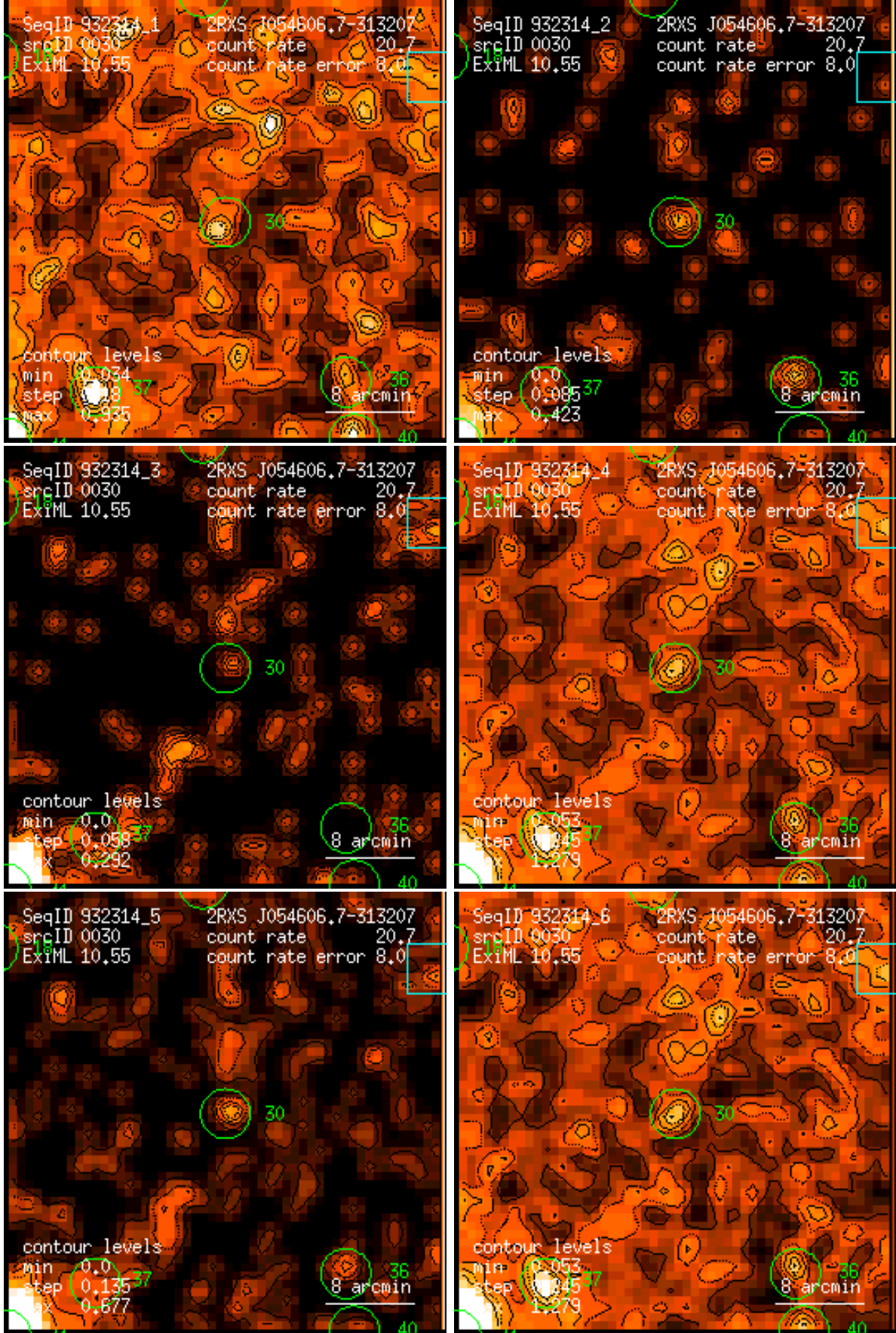
Figure 30: RASS 932314: detection 0030: band rate images, Gaussian filter: (1) PSPC channels 11 – 41, (2) 52 – 90, (3) 91 – 201, (4) 11 – 235, (5) 52 – 201, (6) 11 – 201. Broad band rates in counts/ks. Band rate contour levels in counts/ks/arcmin 2 .
