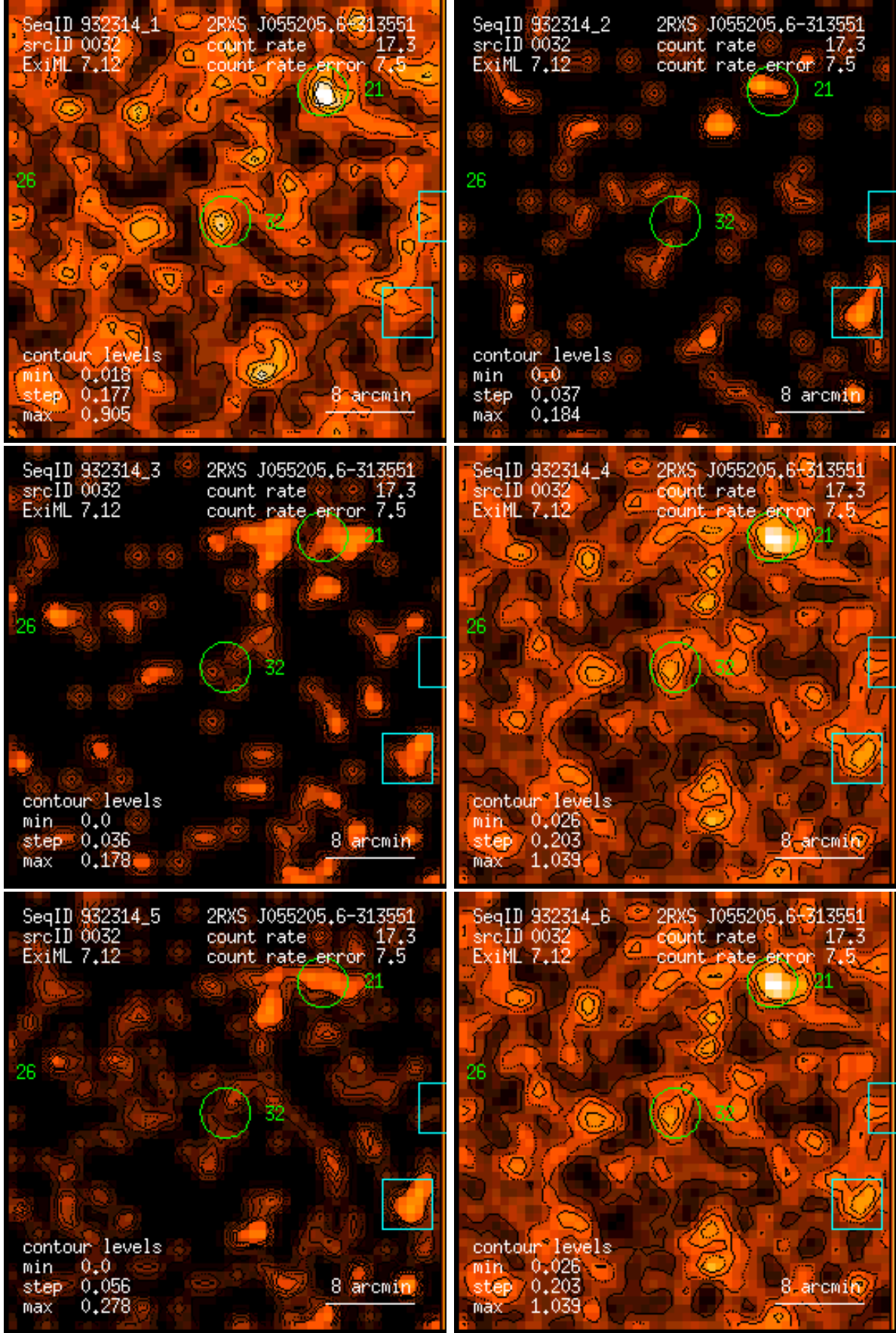
Figure 32: RASS 932314: detection 0032: band rate images, Gaussian filter: (1) PSPC channels 11 – 41, (2) 52 – 90, (3) 91 – 201, (4) 11 – 235, (5) 52 – 201, (6) 11 – 201. Broad band rates in counts/ks. Band rate contour levels in counts/ks/arcmin 2 .
