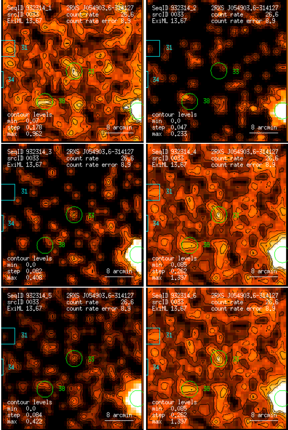
Figure 33: RASS 932314: detection 0033: band rate images, Gaussian filter: (1) PSPC channels 11 – 41, (2) 52 – 90, (3) 91 – 201, (4) 11 – 235, (5) 52 – 201, (6) 11 – 201. Broad band rates in counts/ks. Band rate contour levels in counts/ks/arcmin 2 .
