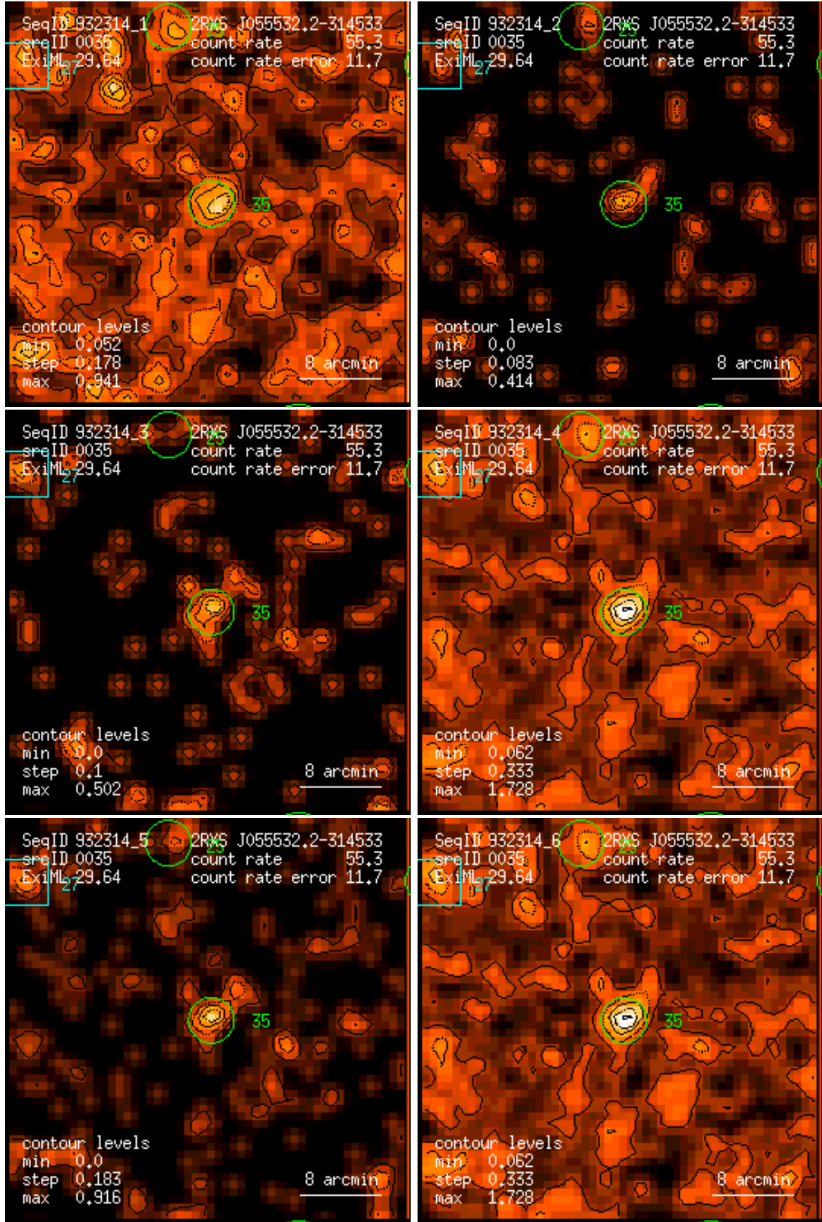
Figure 35: RASS 932314: detection 0035: band rate images, Gaussian filter: (1) PSPC channels 11 – 41, (2) 52 – 90, (3) 91 – 201, (4) 11 – 235, (5) 52 – 201, (6) 11 – 201. Broad band rates in counts/ks. Band rate contour levels in counts/ks/arcmin 2 .
