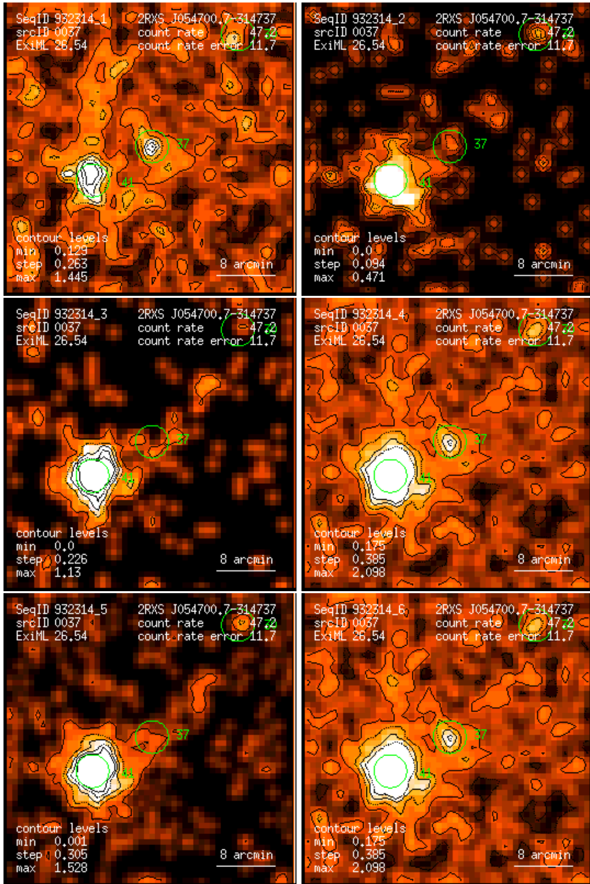
Figure 37: RASS 932314: detection 0037: band rate images, Gaussian filter: (1) PSPC channels 11 – 41, (2) 52 – 90, (3) 91 – 201, (4) 11 – 235, (5) 52 – 201, (6) 11 – 201. Broad band rates in counts/ks. Band rate contour levels in counts/ks/arcmin 2 .
