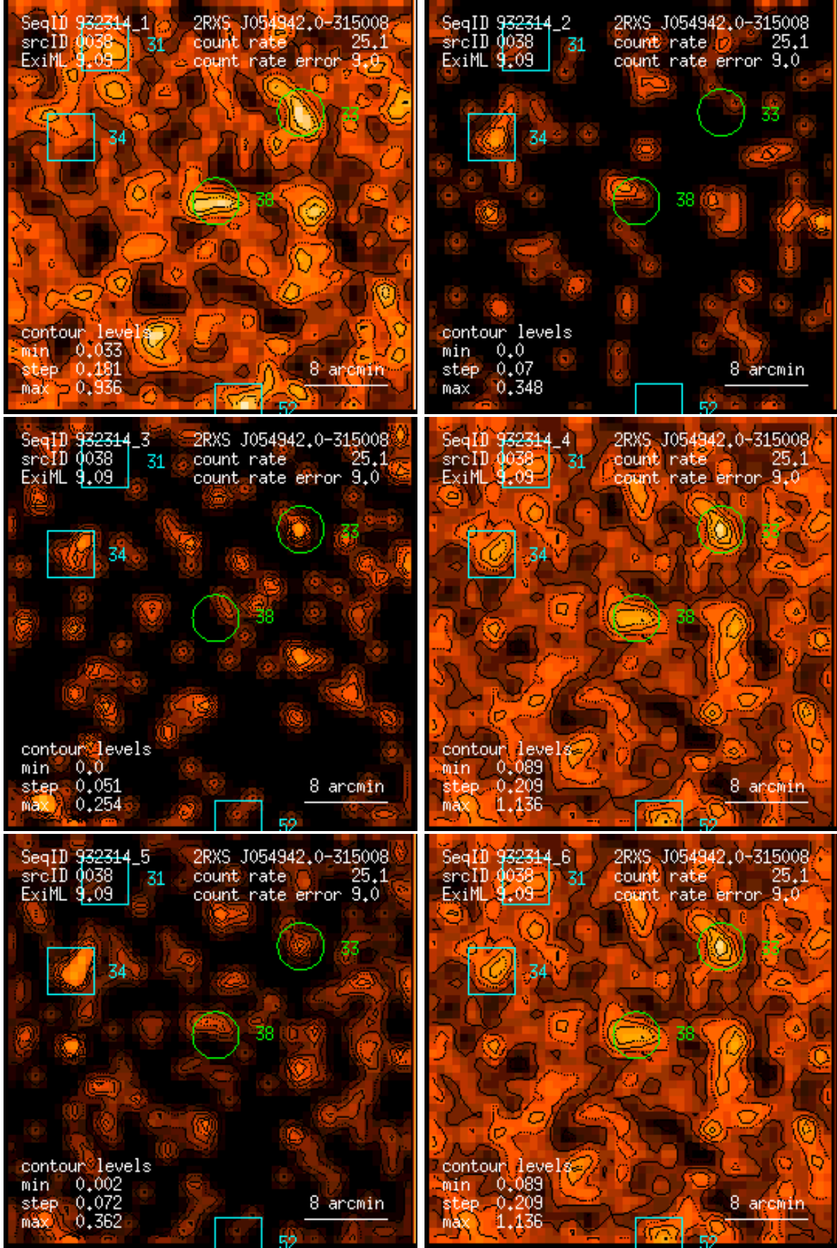
Figure 38: RASS 932314: detection 0038: band rate images, Gaussian filter: (1) PSPC channels 11 – 41, (2) 52 – 90, (3) 91 – 201, (4) 11 – 235, (5) 52 – 201, (6) 11 – 201. Broad band rates in counts/ks. Band rate contour levels in counts/ks/arcmin 2 .
