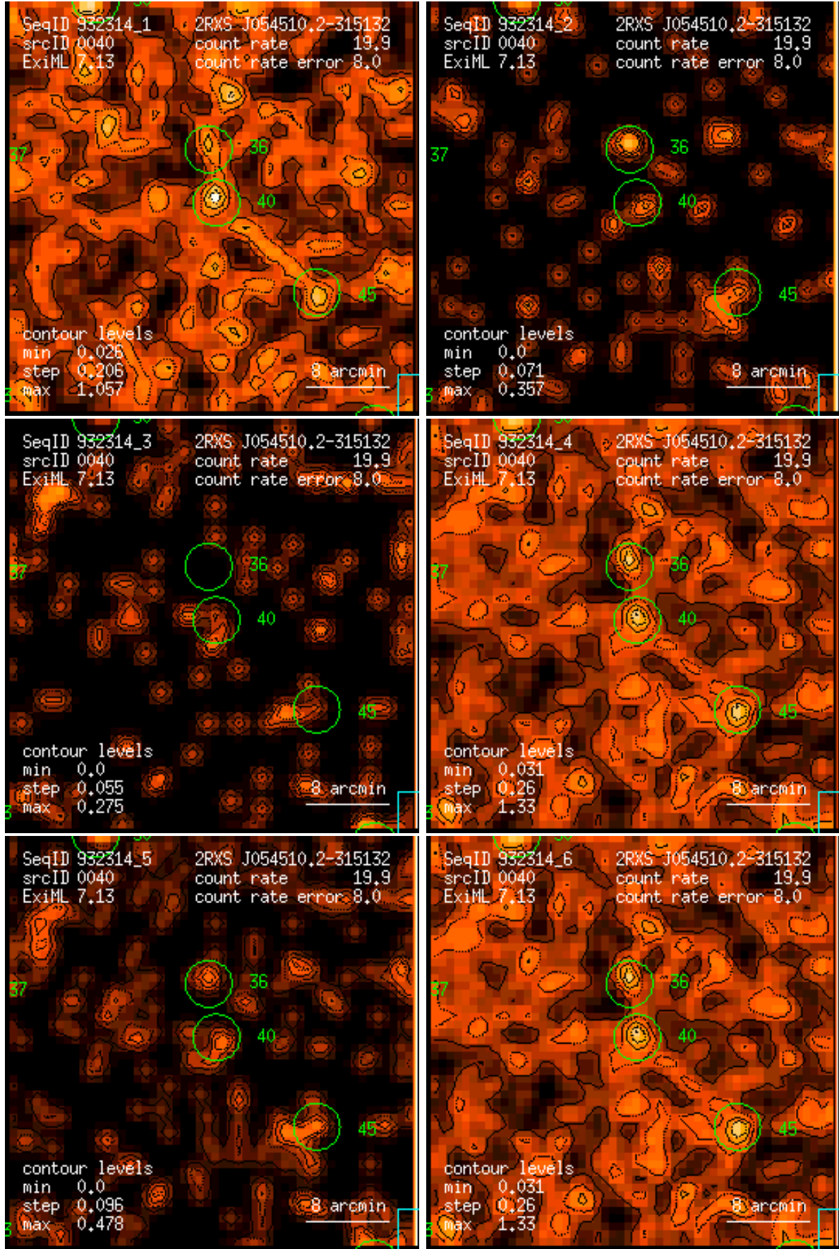
Figure 40: RASS 932314: detection 0040: band rate images, Gaussian filter: (1) PSPC channels 11 – 41, (2) 52 – 90, (3) 91 – 201, (4) 11 – 235, (5) 52 – 201, (6) 11 – 201. Broad band rates in counts/ks. Band rate contour levels in counts/ks/arcmin 2 .
