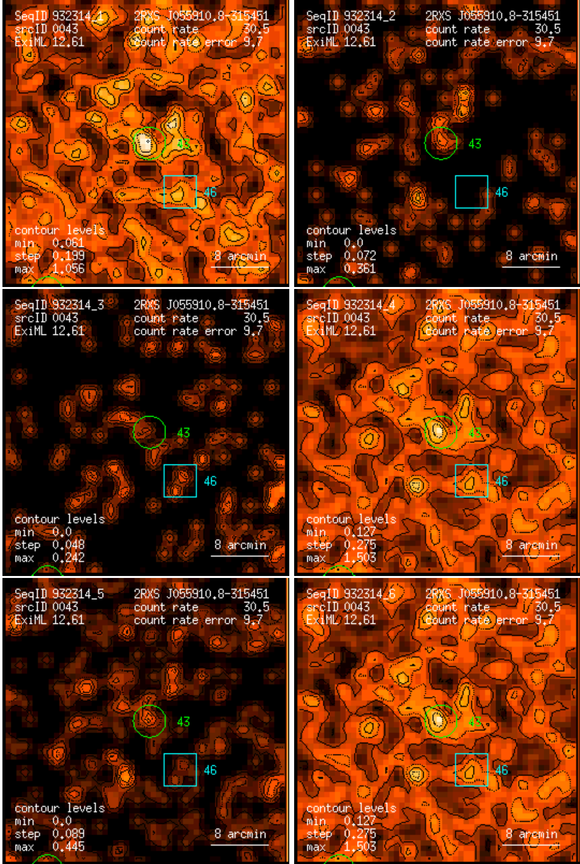
Figure 43: RASS 932314: detection 0043: band rate images, Gaussian filter: (1) PSPC channels 11 – 41, (2) 52 – 90, (3) 91 – 201, (4) 11 – 235, (5) 52 – 201, (6) 11 – 201. Broad band rates in counts/ks. Band rate contour levels in counts/ks/arcmin 2 .
