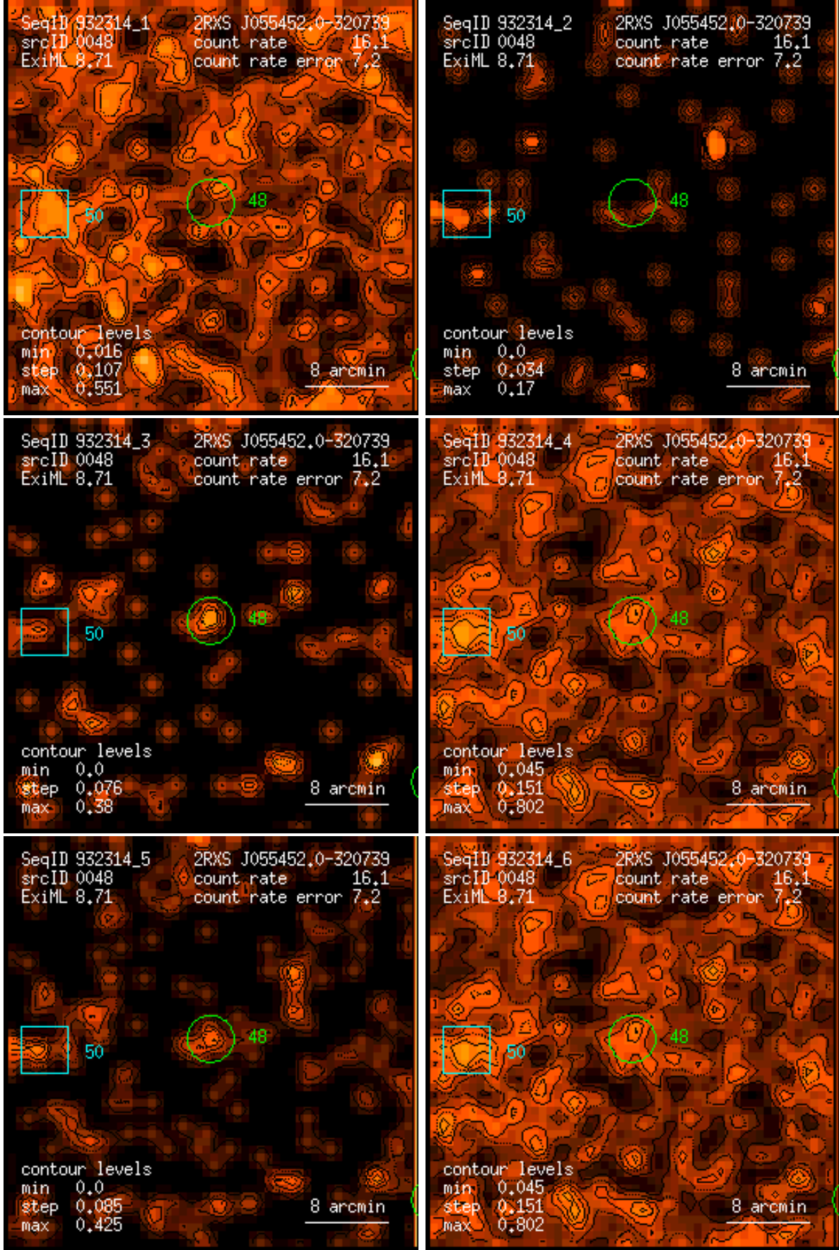
Figure 48: RASS 932314: detection 0048: band rate images, Gaussian filter: (1) PSPC channels 11 – 41, (2) 52 – 90, (3) 91 – 201, (4) 11 – 235, (5) 52 – 201, (6) 11 – 201. Broad band rates in counts/ks. Band rate contour levels in counts/ks/arcmin 2 .
