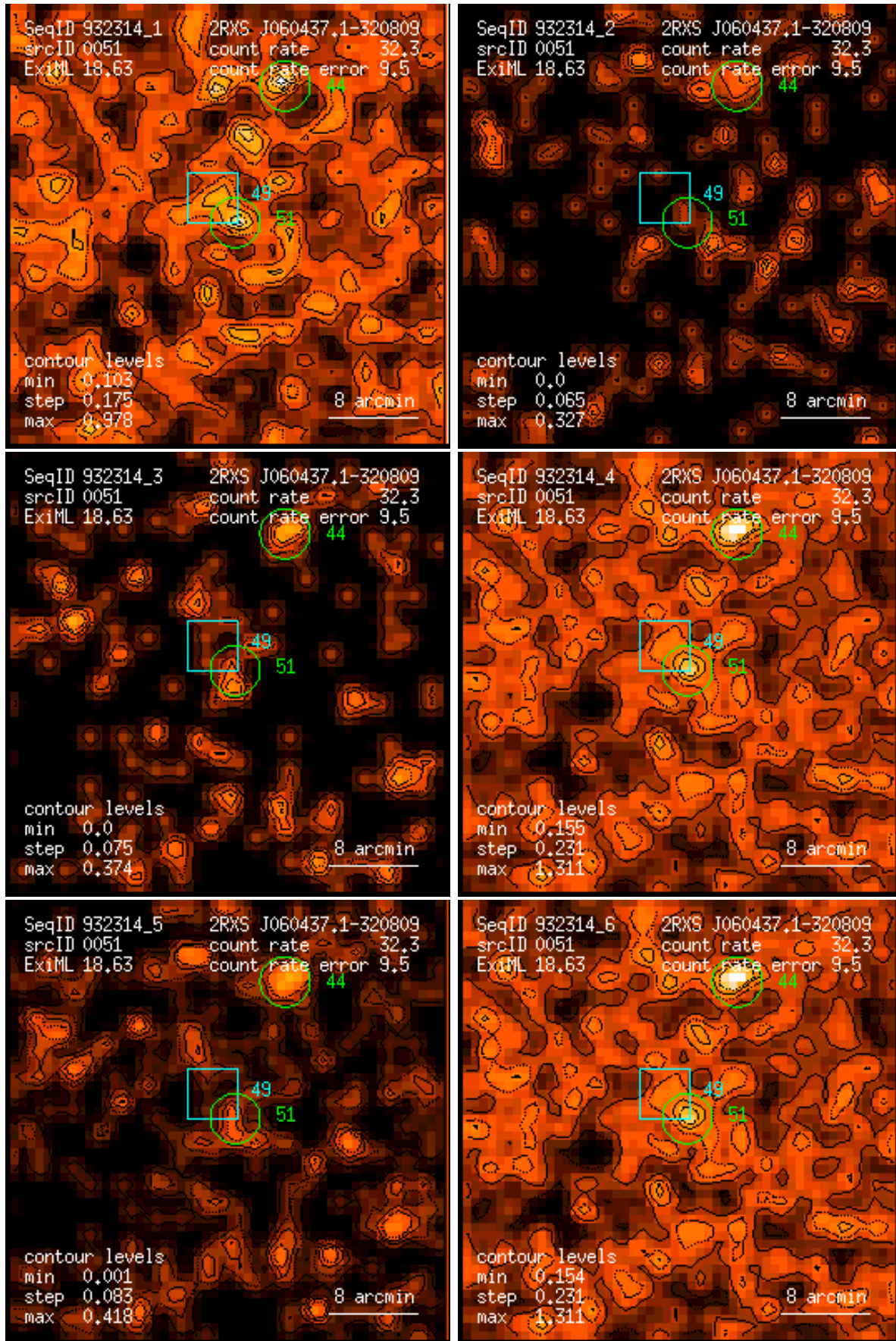
Figure 51: RASS 932314: detection 0051: band rate images, Gaussian filter: (1) PSPC channels 11 – 41, (2) 52 – 90, (3) 91 – 201, (4) 11 – 235, (5) 52 – 201, (6) 11 – 201. Broad band rates in counts/ks. Band rate contour levels in counts/ks/arcmin 2 .
