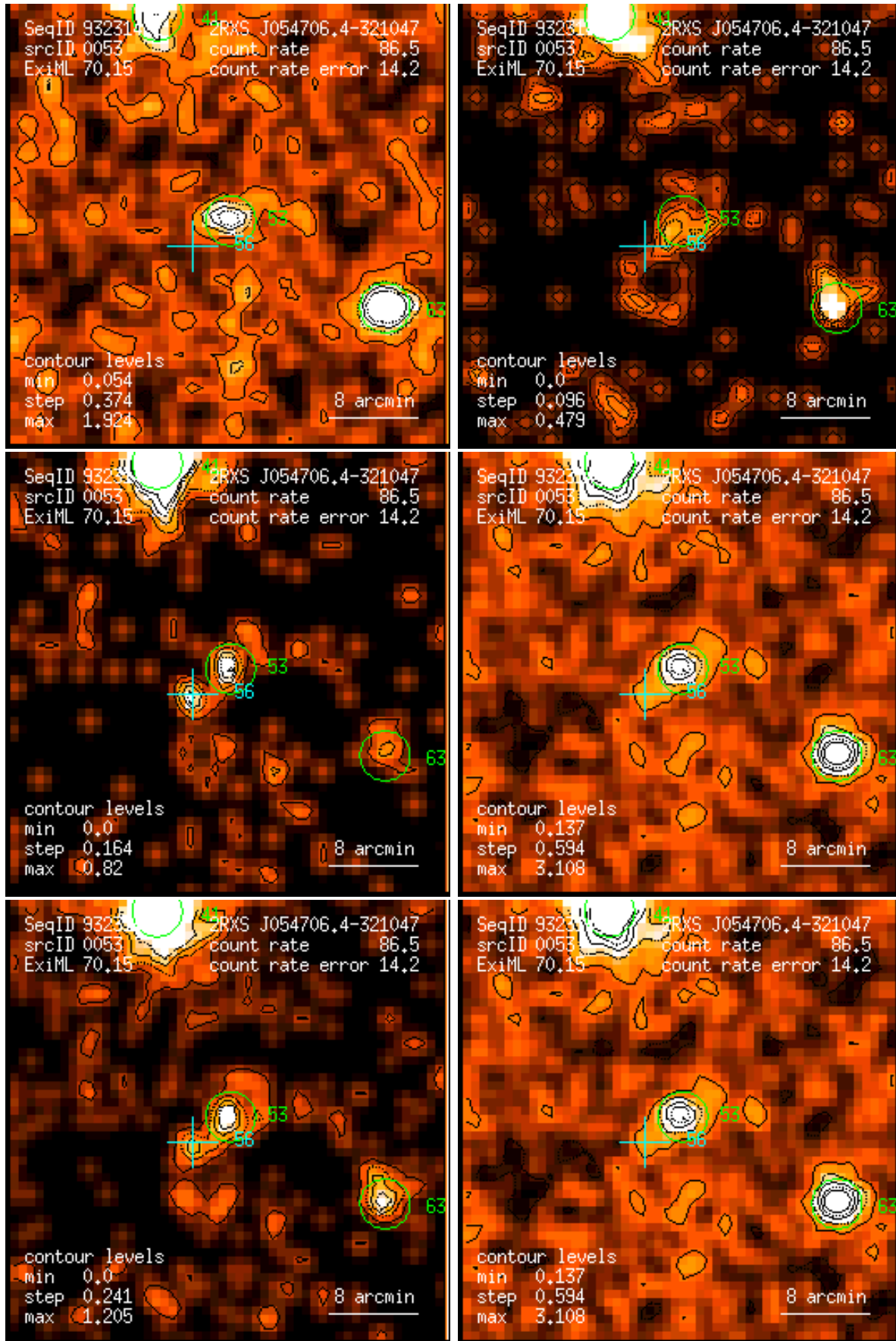
Figure 53: RASS 932314: detection 0053: band rate images, Gaussian filter: (1) PSPC channels 11 – 41, (2) 52 – 90, (3) 91 – 201, (4) 11 – 235, (5) 52 – 201, (6) 11 – 201. Broad band rates in counts/ks. Band rate contour levels in counts/ks/arcmin 2 .
