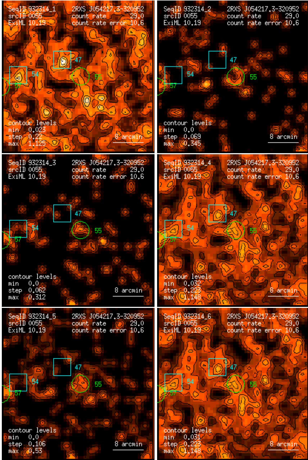
Figure 55: RASS 932314: detection 0055: band rate images, Gaussian filter: (1) PSPC channels 11 – 41, (2) 52 – 90, (3) 91 – 201, (4) 11 – 235, (5) 52 – 201, (6) 11 – 201. Broad band rates in counts/ks. Band rate contour levels in counts/ks/arcmin 2 .
