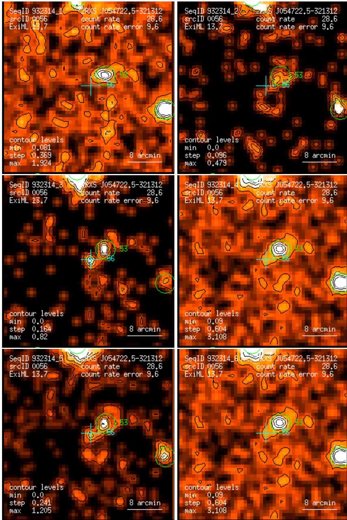
Figure 56: RASS 932314: detection 0056: band rate images, Gaussian filter: (1) PSPC channels 11 – 41, (2) 52 – 90, (3) 91 – 201, (4) 11 – 235, (5) 52 – 201, (6) 11 – 201. Broad band rates in counts/ks. Band rate contour levels in counts/ks/arcmin 2 .
