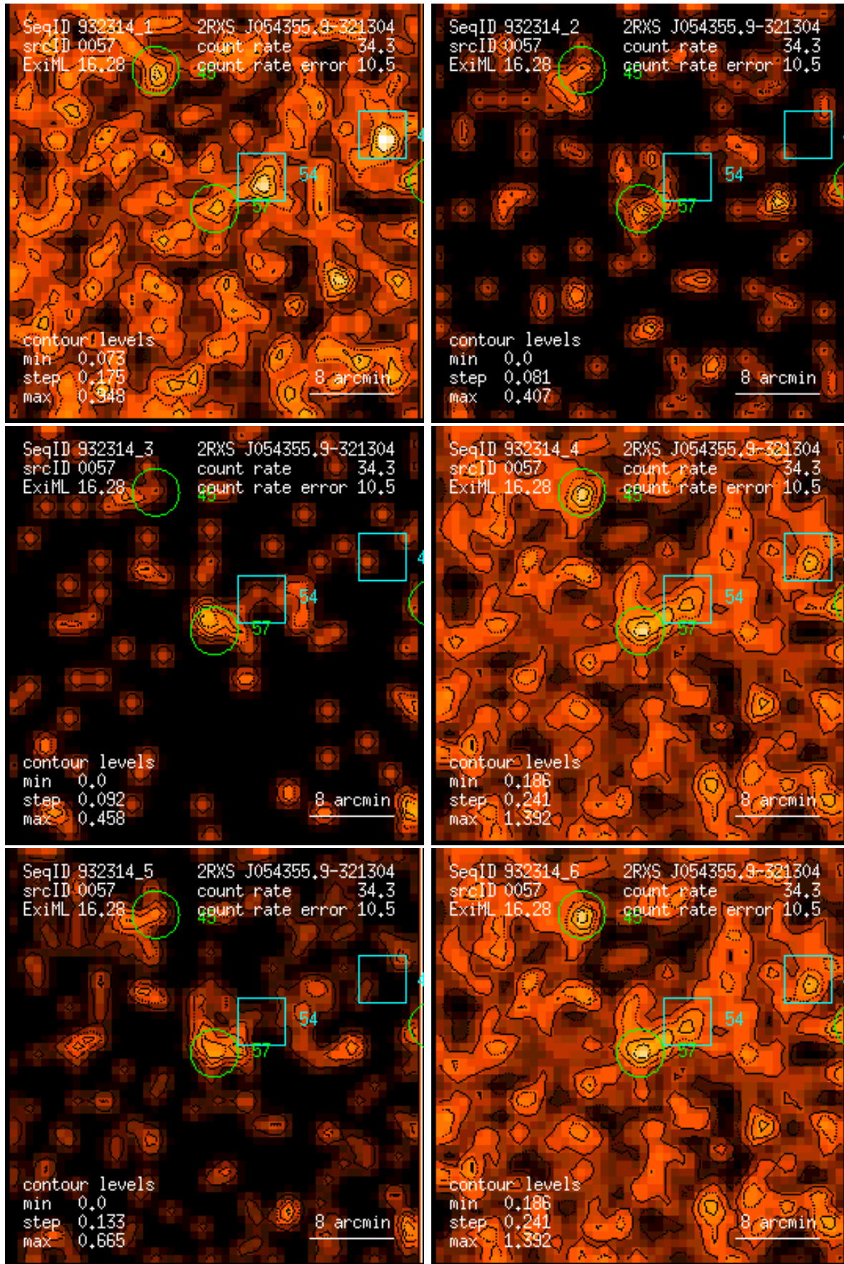
Figure 57: RASS 932314: detection 0057: band rate images, Gaussian filter: (1) PSPC channels 11 – 41, (2) 52 – 90, (3) 91 – 201, (4) 11 – 235, (5) 52 – 201, (6) 11 – 201. Broad band rates in counts/ks. Band rate contour levels in counts/ks/arcmin 2 .
