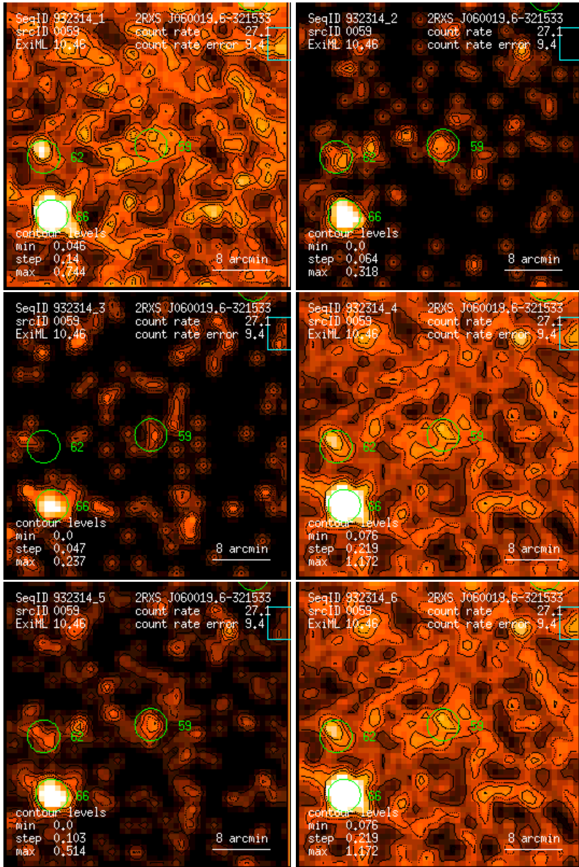
Figure 59: RASS 932314: detection 0059: band rate images, Gaussian filter: (1) PSPC channels 11 – 41, (2) 52 – 90, (3) 91 – 201, (4) 11 – 235, (5) 52 – 201, (6) 11 – 201. Broad band rates in counts/ks. Band rate contour levels in counts/ks/arcmin 2 .
