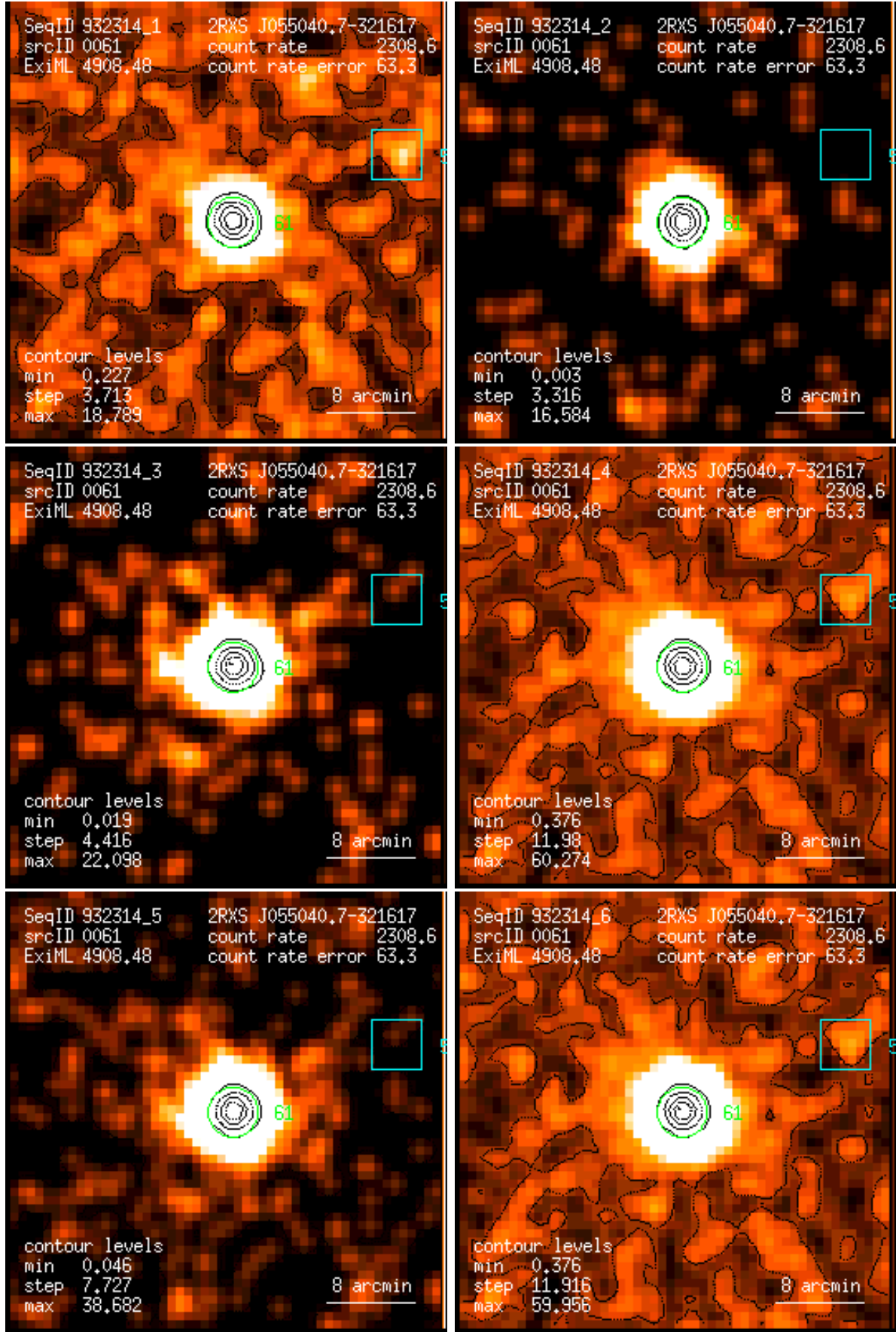
Figure 61: RASS 932314: detection 0061: band rate images, Gaussian filter: (1) PSPC channels 11 – 41, (2) 52 – 90, (3) 91 – 201, (4) 11 – 235, (5) 52 – 201, (6) 11 – 201. Broad band rates in counts/ks. Band rate contour levels in counts/ks/arcmin 2 .
