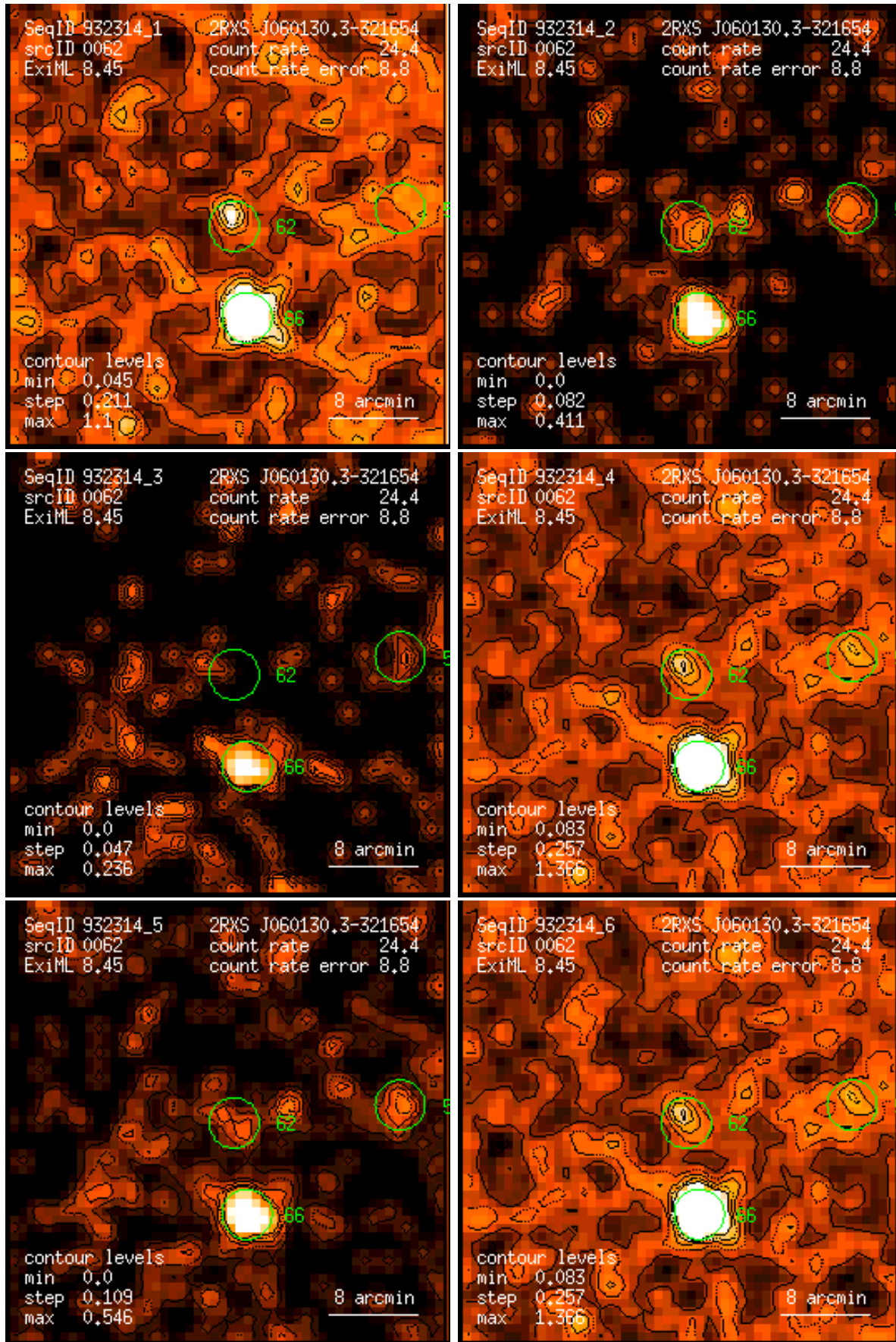
Figure 62: RASS 932314: detection 0062: band rate images, Gaussian filter: (1) PSPC channels 11 – 41, (2) 52 – 90, (3) 91 – 201, (4) 11 – 235, (5) 52 – 201, (6) 11 – 201. Broad band rates in counts/ks. Band rate contour levels in counts/ks/arcmin 2 .
