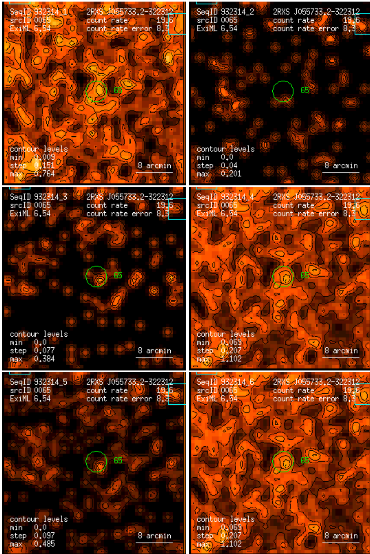
Figure 65: RASS 932314: detection 0065: band rate images, Gaussian filter: (1) PSPC channels 11 – 41, (2) 52 – 90, (3) 91 – 201, (4) 11 – 235, (5) 52 – 201, (6) 11 – 201. Broad band rates in counts/ks. Band rate contour levels in counts/ks/arcmin 2 .
