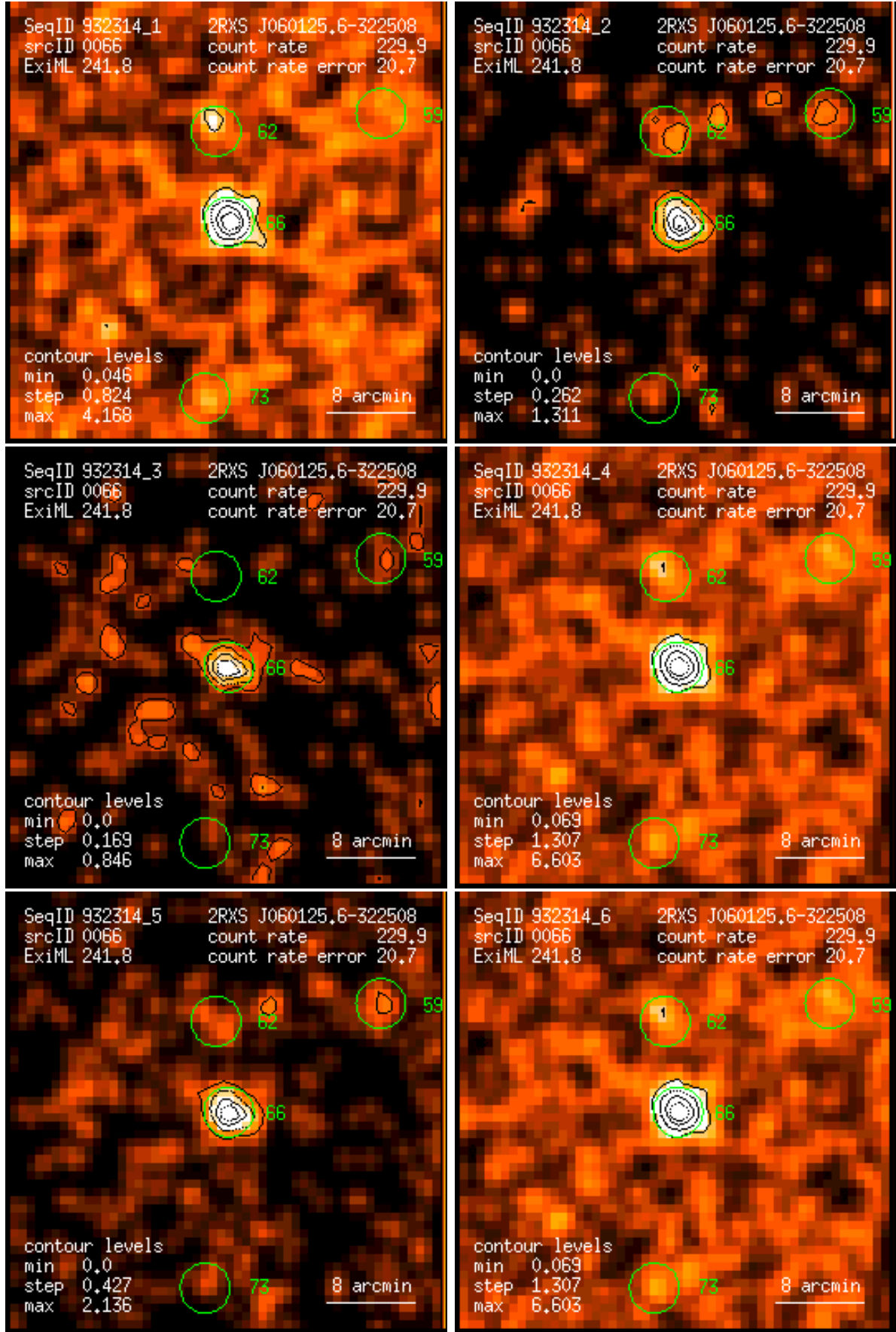
Figure 66: RASS 932314: detection 0066: band rate images, Gaussian filter: (1) PSPC channels 11 – 41, (2) 52 – 90, (3) 91 – 201, (4) 11 – 235, (5) 52 – 201, (6) 11 – 201. Broad band rates in counts/ks. Band rate contour levels in counts/ks/arcmin 2 .
