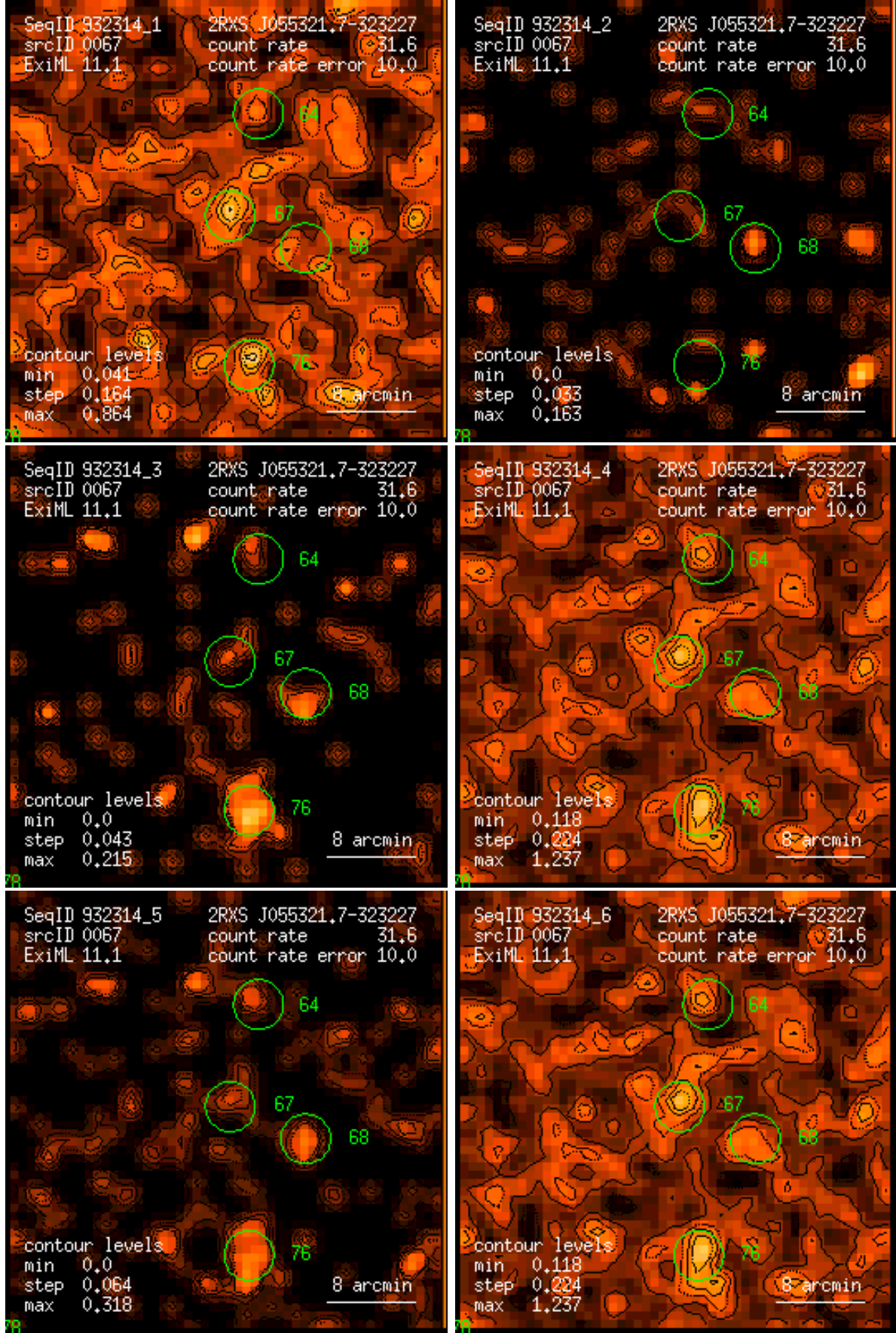
Figure 67: RASS 932314: detection 0067: band rate images, Gaussian filter: (1) PSPC channels 11 – 41, (2) 52 – 90, (3) 91 – 201, (4) 11 – 235, (5) 52 – 201, (6) 11 – 201. Broad band rates in counts/ks. Band rate contour levels in counts/ks/arcmin 2 .
