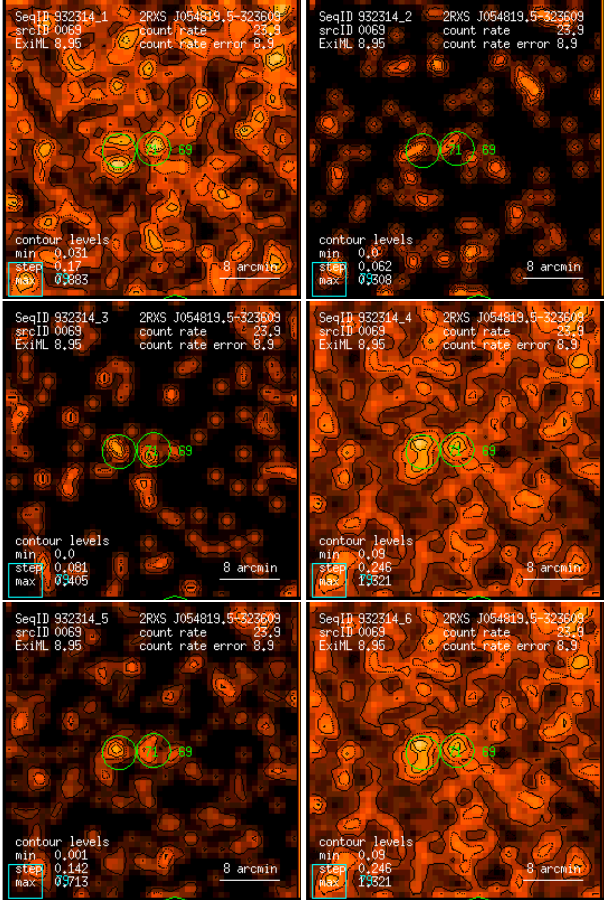
Figure 69: RASS 932314: detection 0069: band rate images, Gaussian filter: (1) PSPC channels 11 – 41, (2) 52 – 90, (3) 91 – 201, (4) 11 – 235, (5) 52 – 201, (6) 11 – 201. Broad band rates in counts/ks. Band rate contour levels in counts/ks/arcmin 2 .
