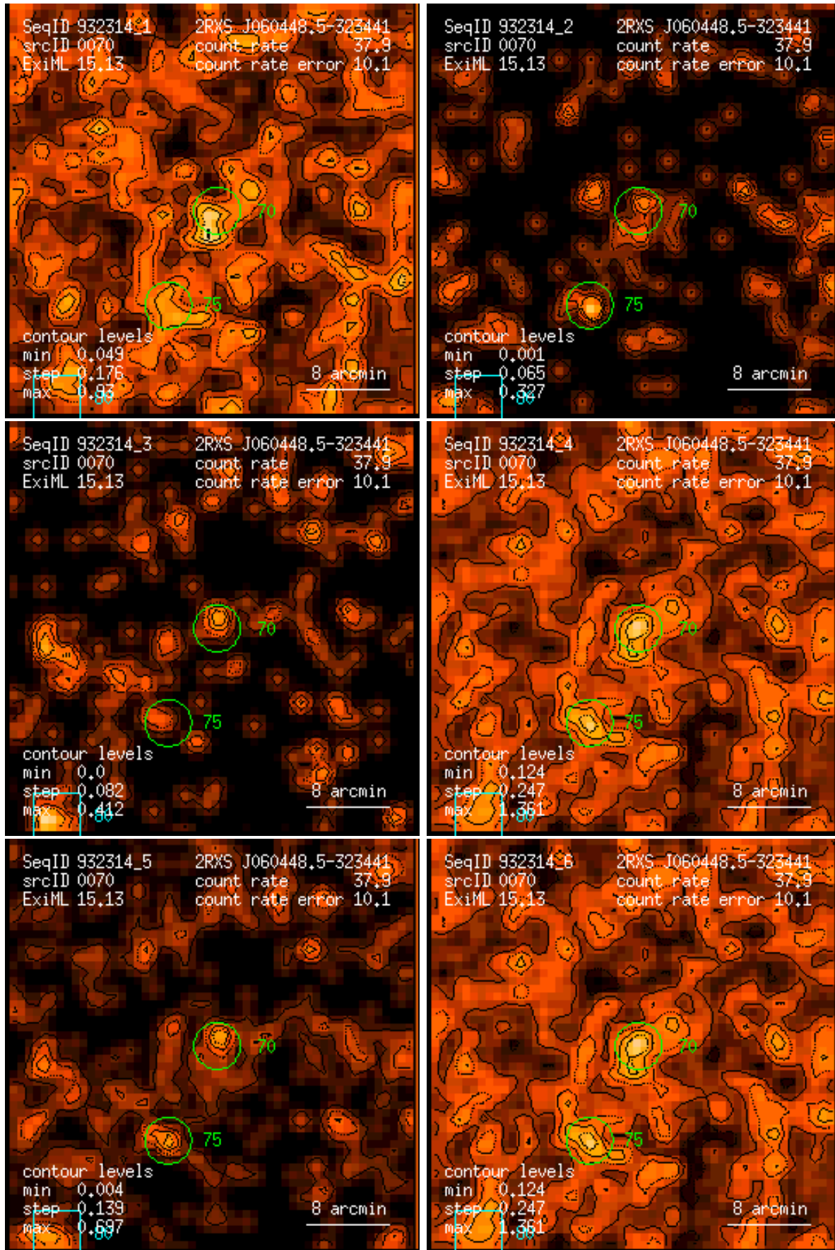
Figure 70: RASS 932314: detection 0070: band rate images, Gaussian filter: (1) PSPC channels 11 – 41, (2) 52 – 90, (3) 91 – 201, (4) 11 – 235, (5) 52 – 201, (6) 11 – 201. Broad band rates in counts/ks. Band rate contour levels in counts/ks/arcmin 2 .
